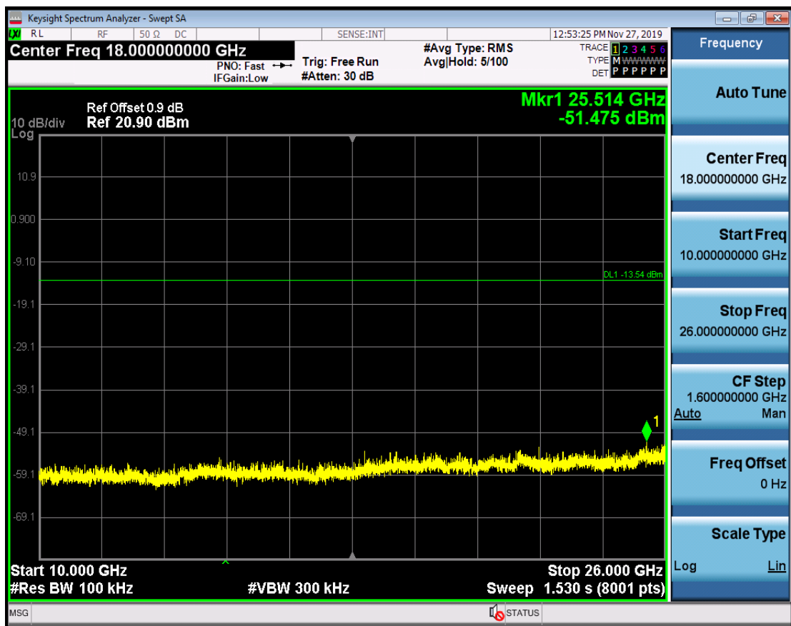
RF Conducted Spurious Emissions_DH5_2441
