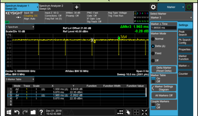
802.11ac-VHT20 (T = 1.930ms)
