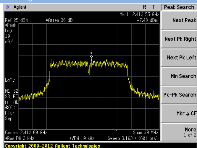
802.11g CHANNEL 1
