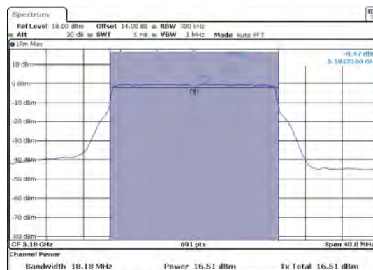
ANT 2(802.11 N20)
