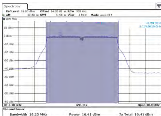
ANT 1(802.11N20)
