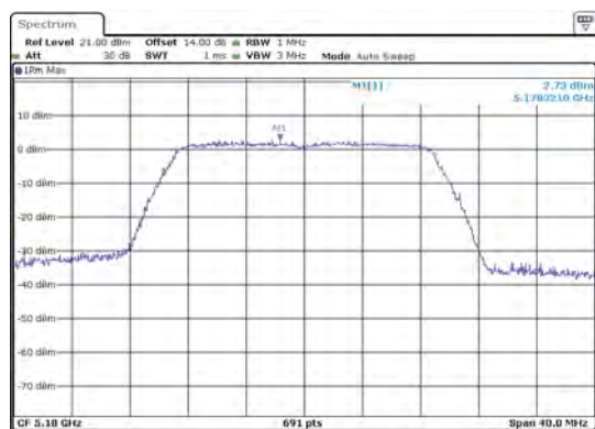
ANT 1(11N20)
