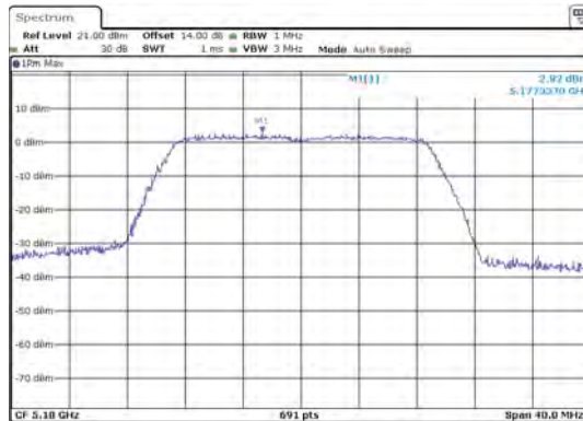
ANT 2(11N20)
