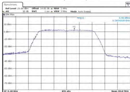
ANT 1(11N20)
