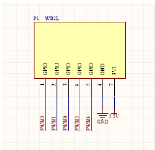
Figure 6-3 WB2L pins
