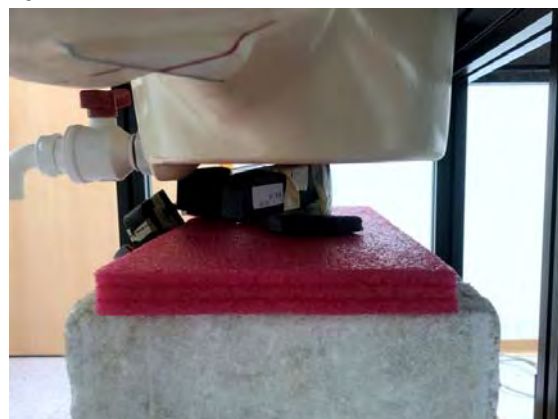
Fig.8 EUT 8 to flat phantom
