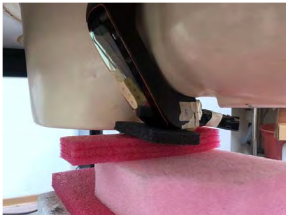
Fig.10 EUT 7 to flat phantom
