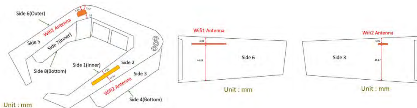
Fig.13 Antenna position of EUT
