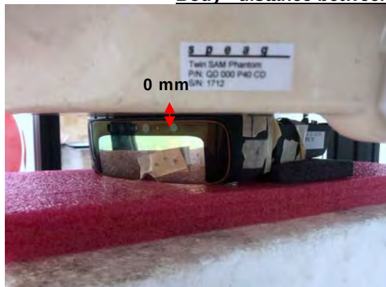
Fig.6 EUT 5 to flat phantom
