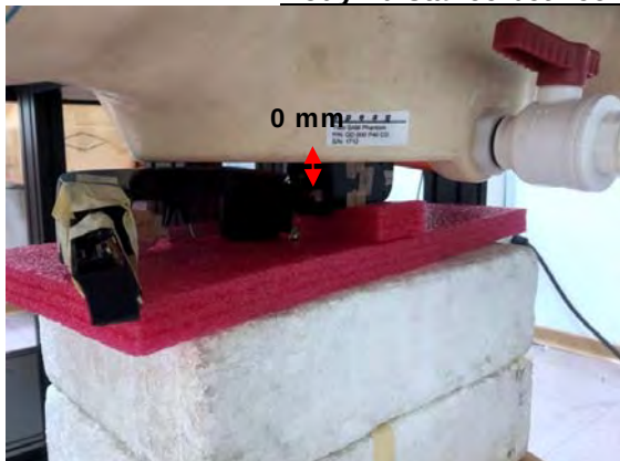
Fig.3 EUT 2 to flat phantom
