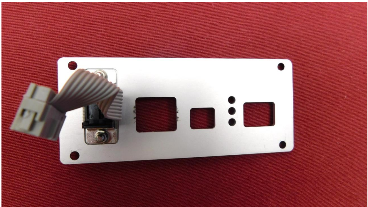
Picture 4: Front plate with RS232 connector, top view
