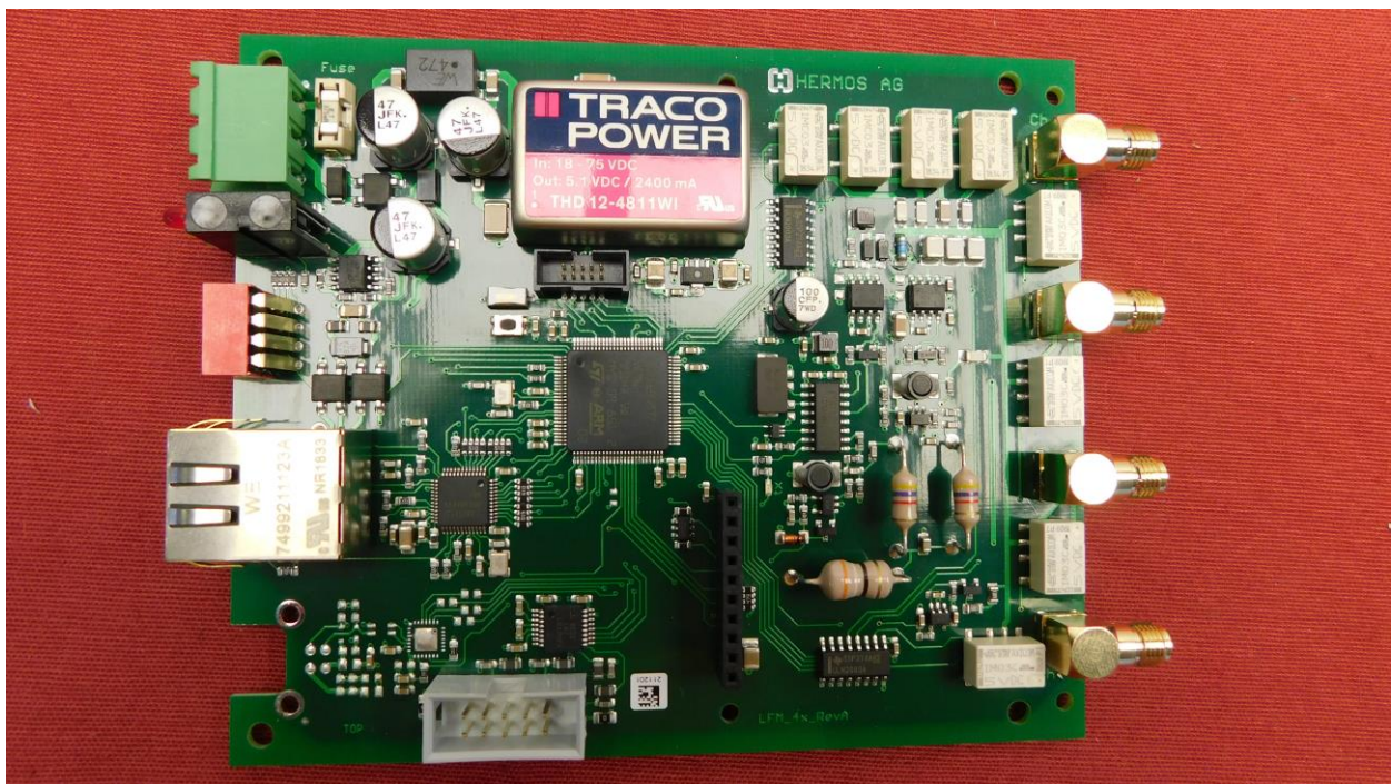
Picture 2: Board, top view
