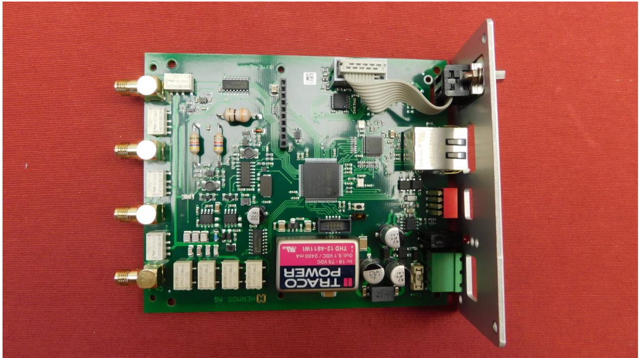
Picture 1: Board with front plate, top view
