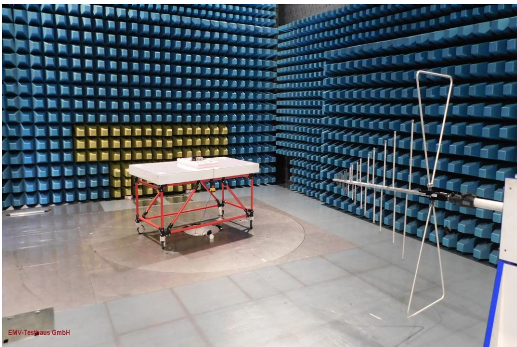
Picture 4: SAC, radiated emission test 30 MHz -1 GHz and bandwidth test (rear view)
