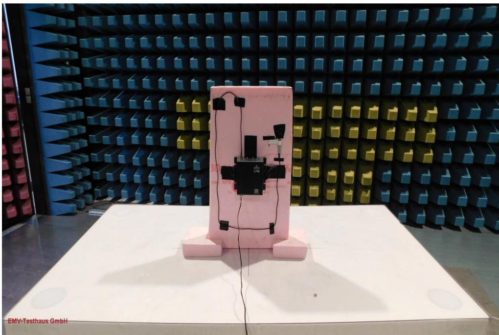
Picture 8: EUT-position Z
