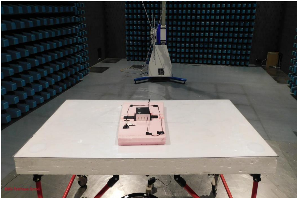
Picture 3: SAC, radiated emission test 30 MHz -1 GHz and bandwidth test (front view)
