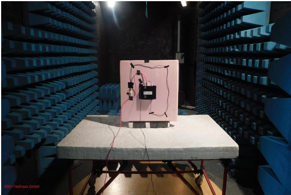
Picture 7: EUT-position Y
