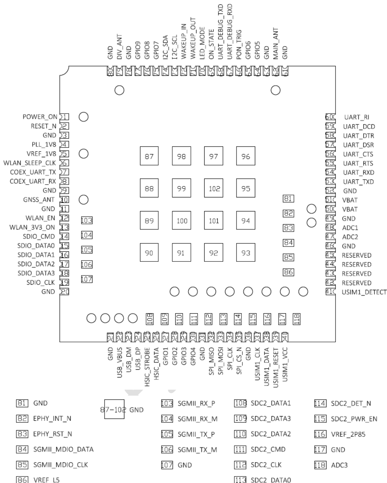
Figure 2-1 Pin Assignment
