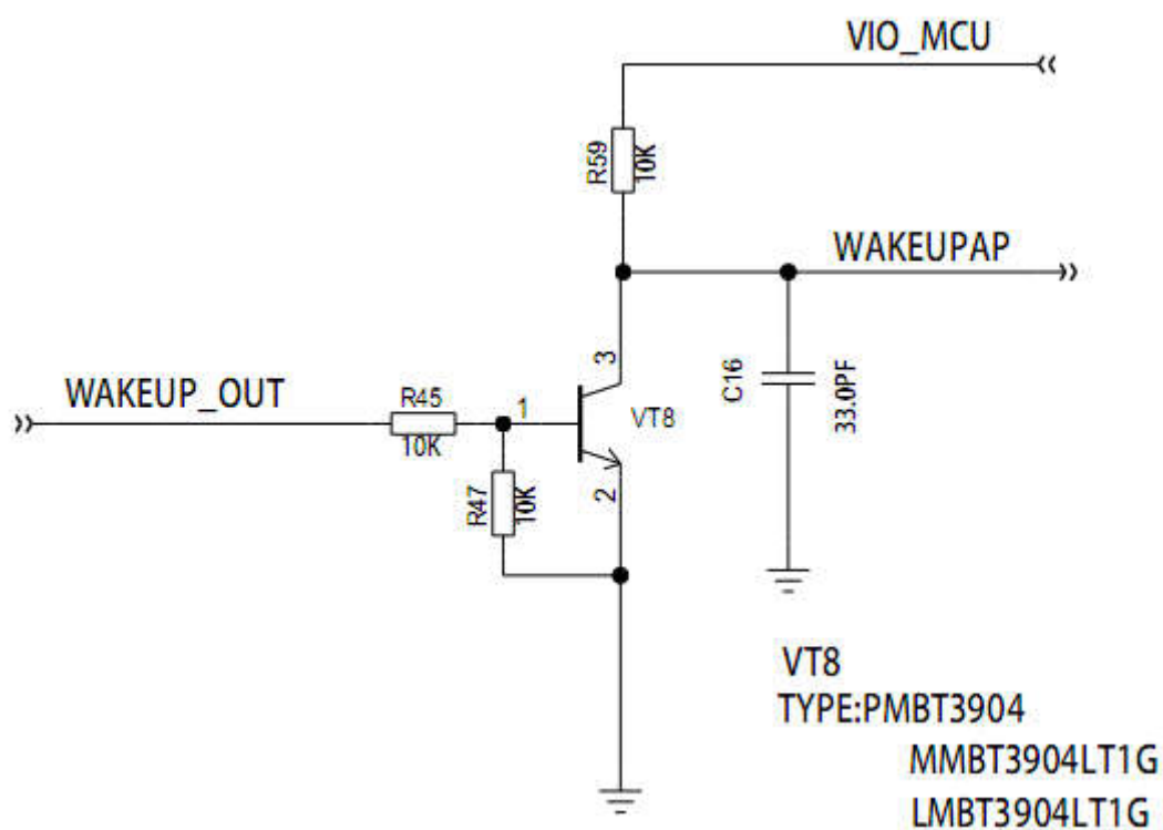
Figure 2-33 WAKEUP_OUTreference design
