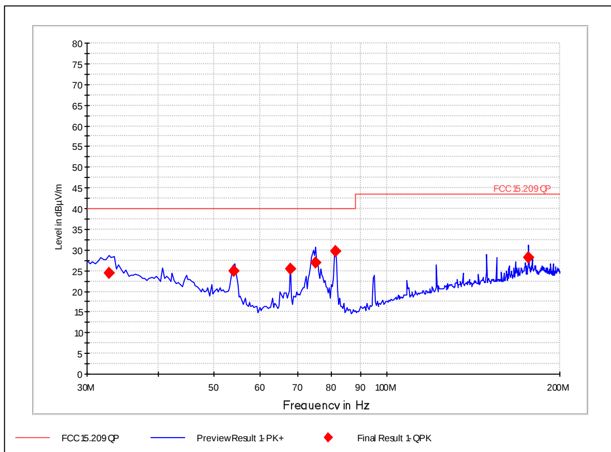
Figure 7. Emission outside frequency band 30 -200 MHz. EUT horizontal.
