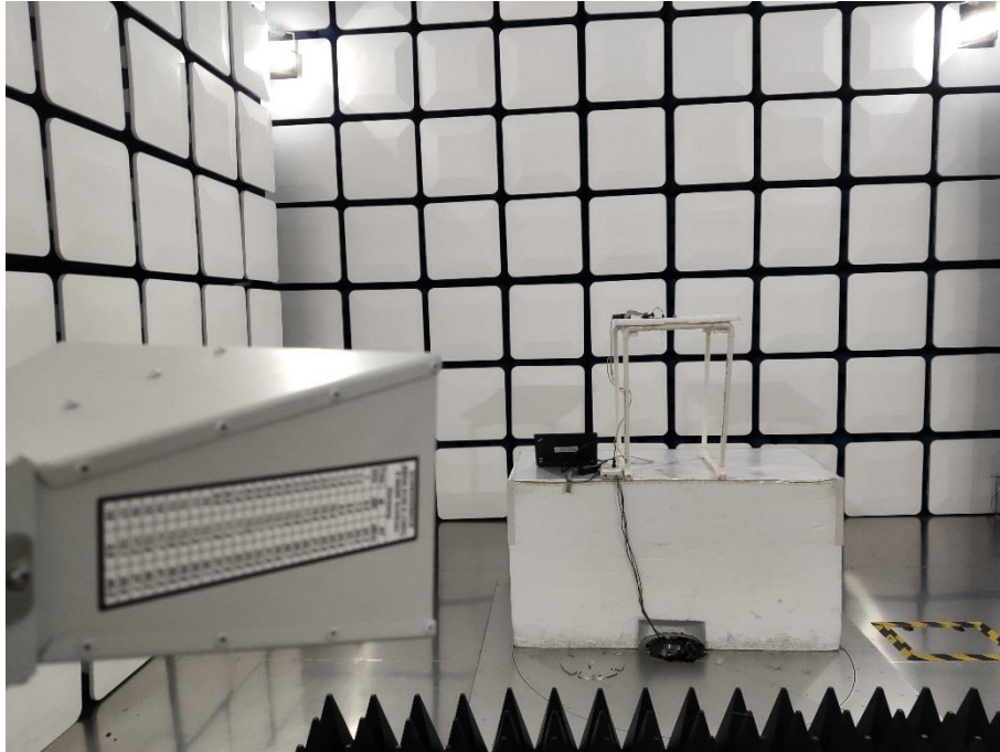
Above 1GHz (External Antenna)
