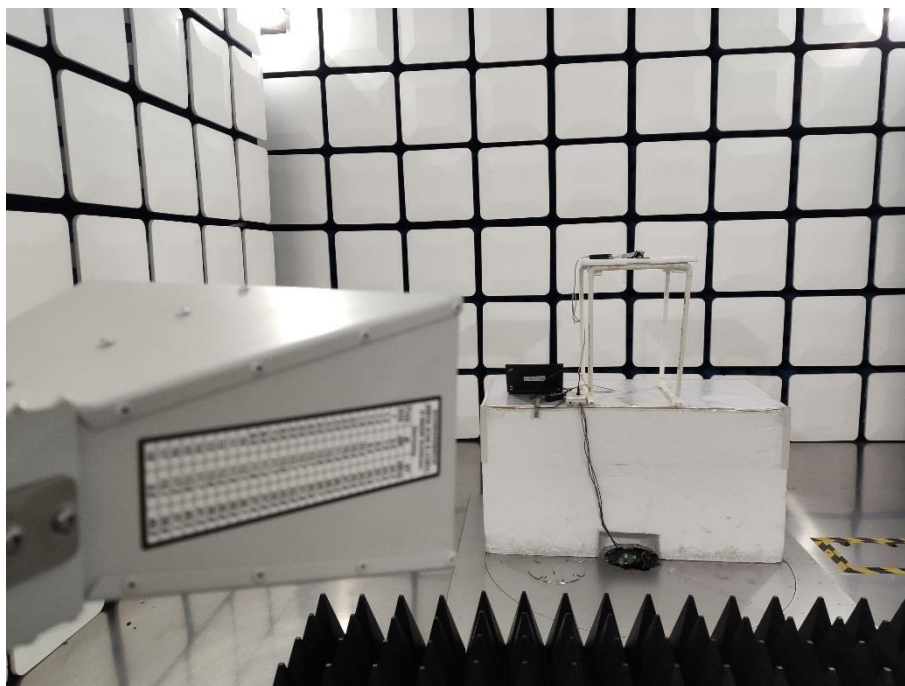
Above 1GHz (Built-in Antenna)
