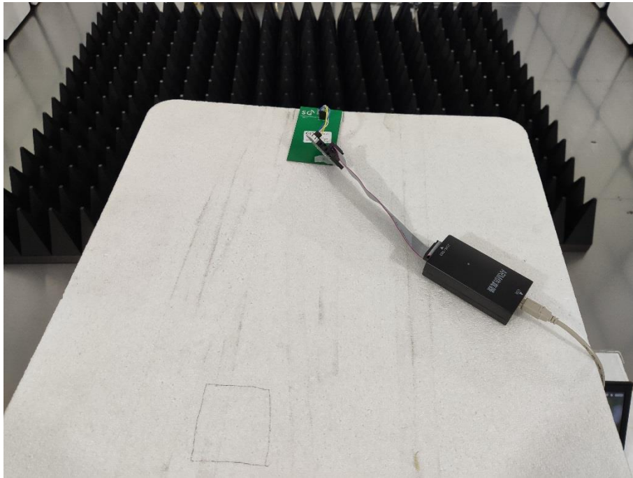
Close-up (Built-in Antenna)
