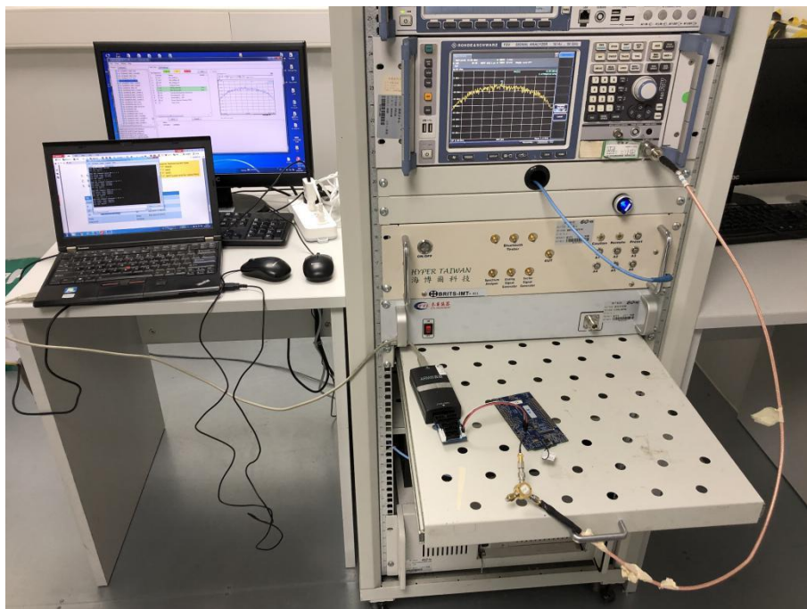
Conducted Test-BLE (External Antenna)
