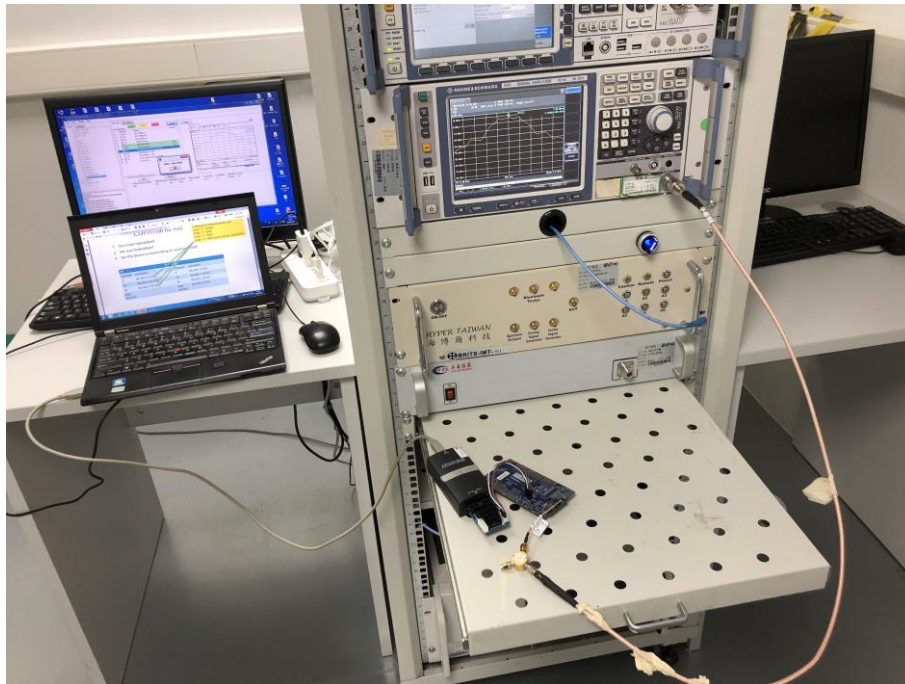
Conducted Test-BLE (Built-in Antenna)
