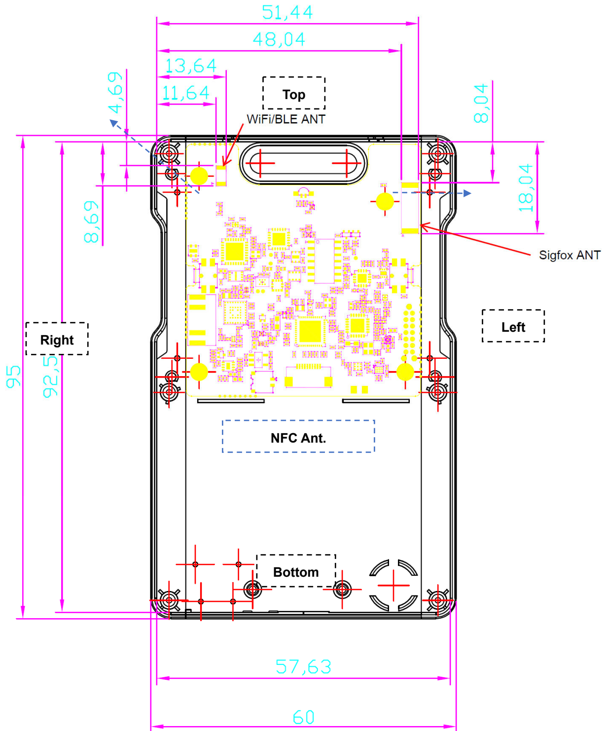
Figure F-1 Antenna Location (Rear Side View)
