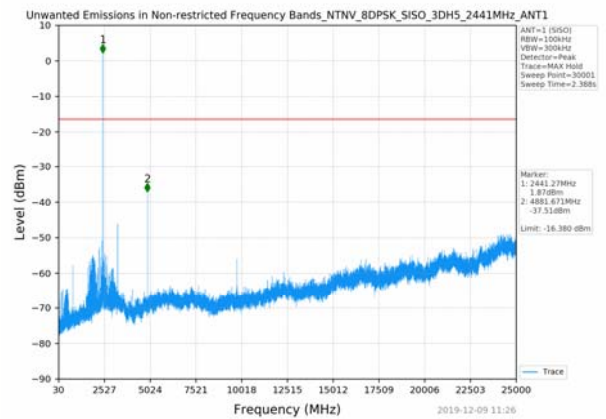
30MHz-25GHz CH39
