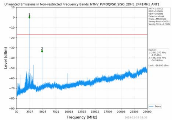
30MHz-25GHz CH39
