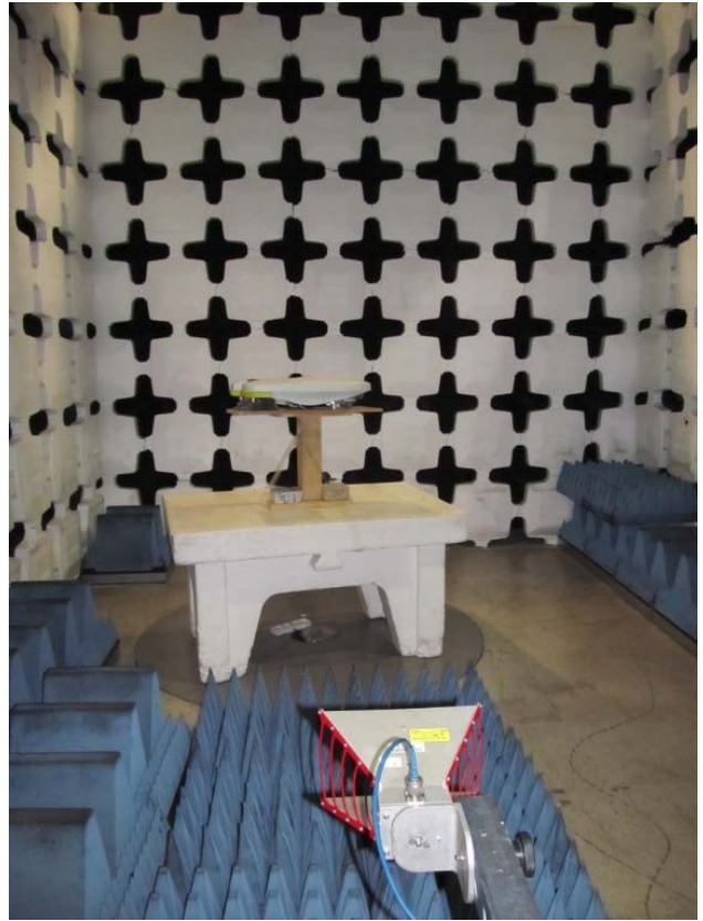
Radiated emissions test setup with Horn antenna.
