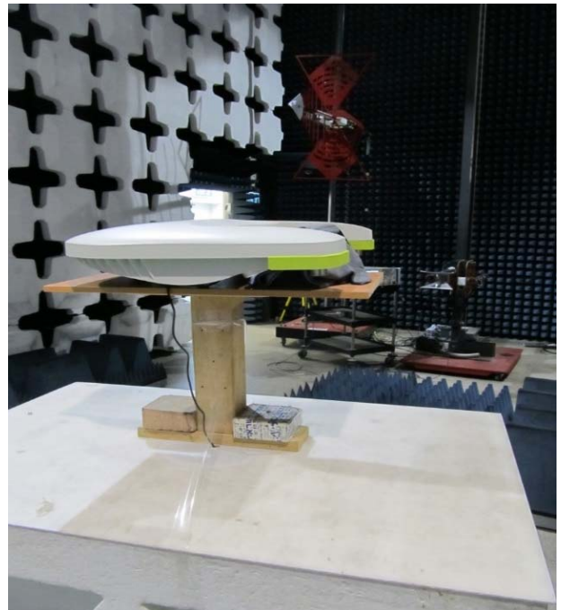
Radiated emissions test setup with Horn antenna.
