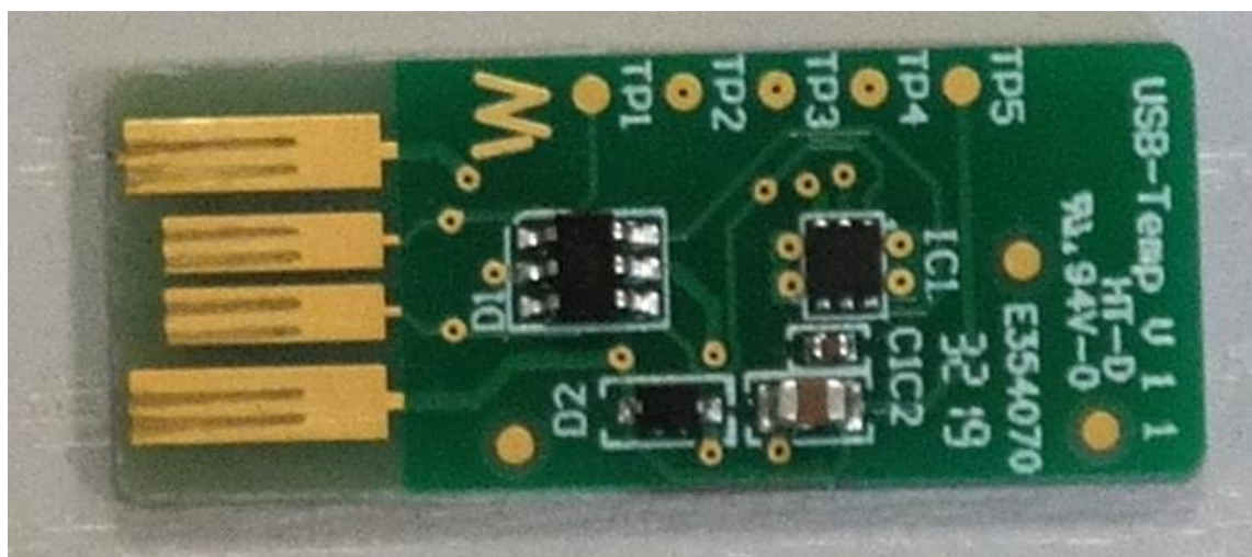
Picture 10: NIST board – top side
