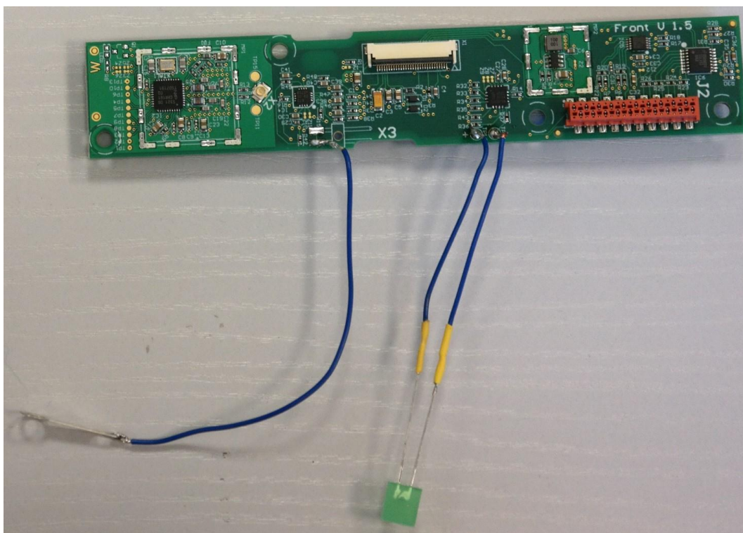
Picture 5: RFID board– top side
