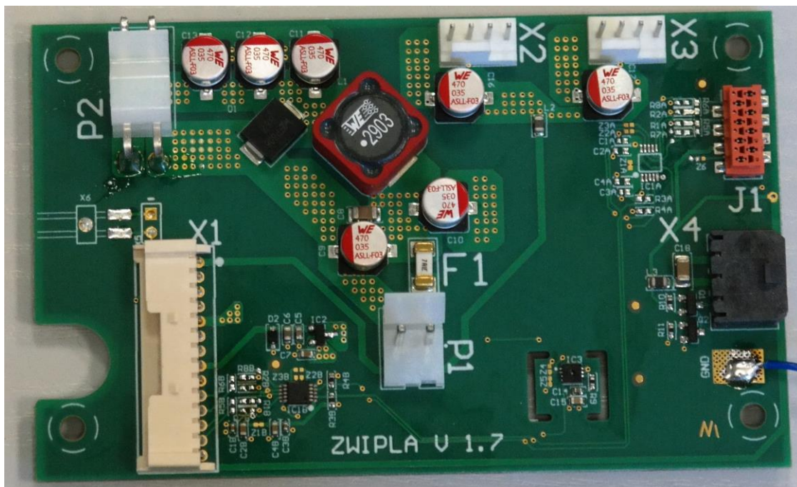
Picture 13: ZWIPLA board – top side
