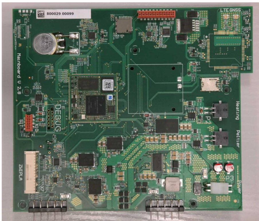
Picture 15: Main board – top side
