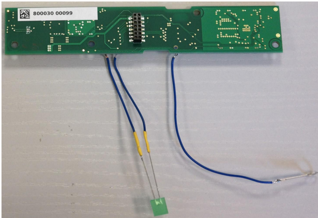
Picture 6: RFID board – bottom side
