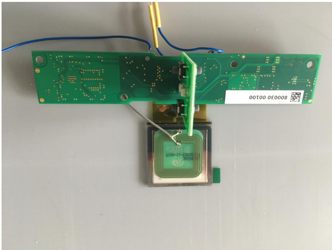
Picture 4: RFID board
