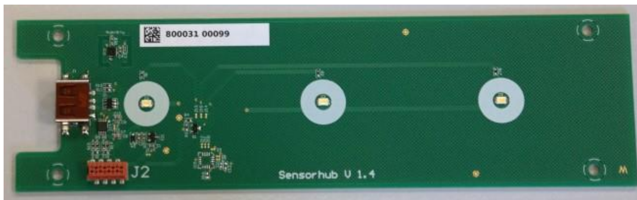
Picture 17: Sensorhub board – top side
