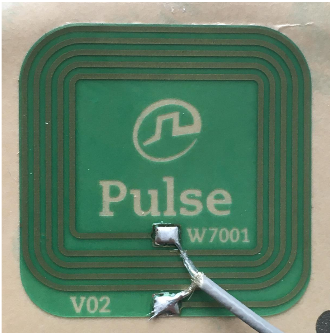
Picture 9: RFID antenna
