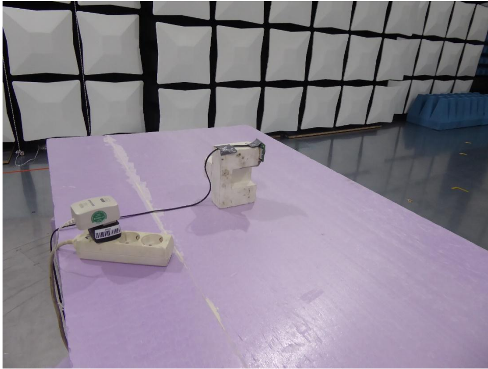
191836_03.JPG: EUT setup
