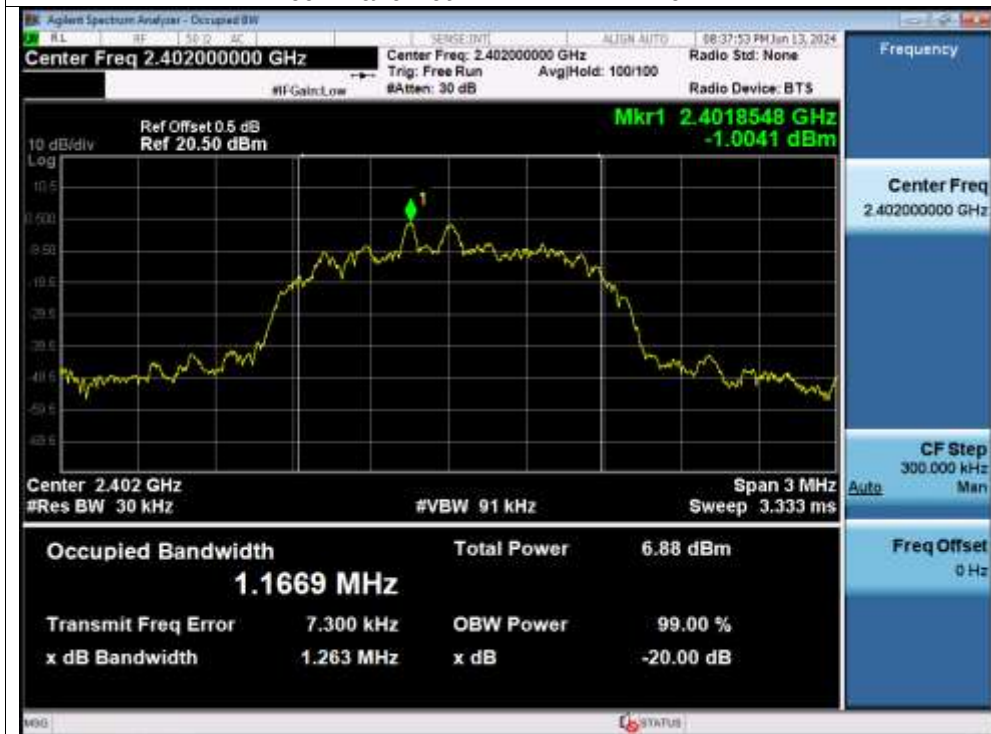
-20dB Bandwidth NVNT 2-DH1 2402MHz
