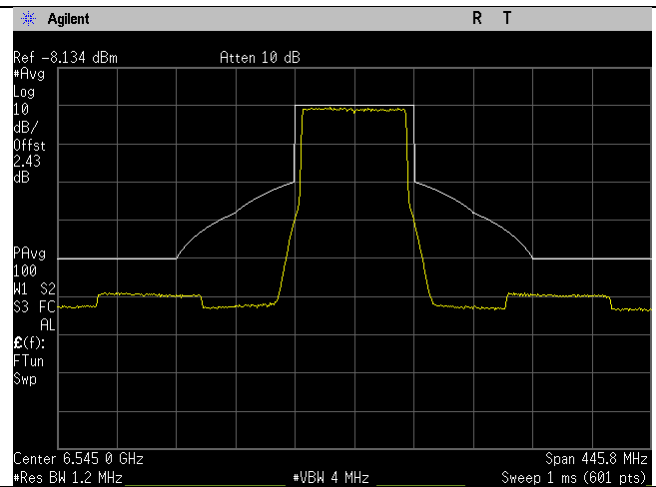
6545MHz_119_80MHz BW_be-mode_Chain 3
