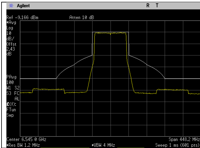
6545MHz_119_80MHz BW_be-mode_Chain 2
