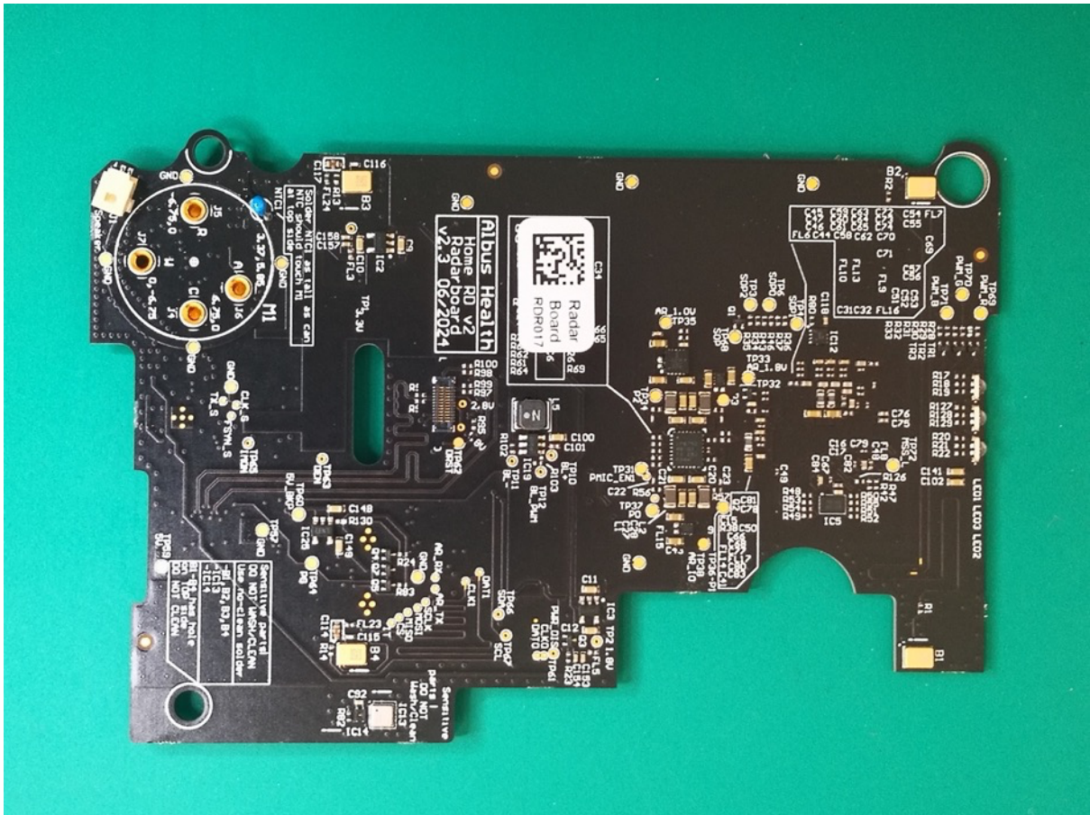
Internal board- Radar Board (bottom):
