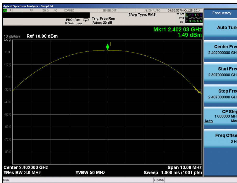
Plot 6-4. Peak Power Plot (Bluetooth (LE) – Ch. 0)
