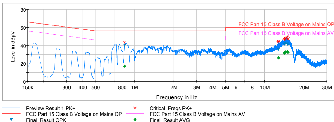
Plot 6-64. Line Conducted Plot with 802.11b (N)
