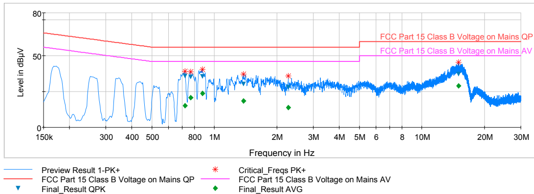
Plot 6-63. Line Conducted Plot with 802.11b (L1)
