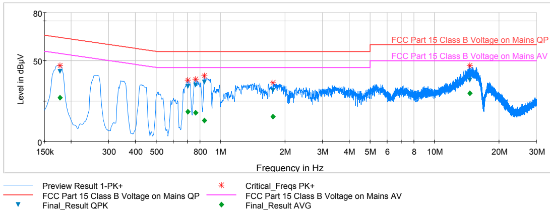
Plot 6-65. Line Conducted Plot with 802.11a (L1)
