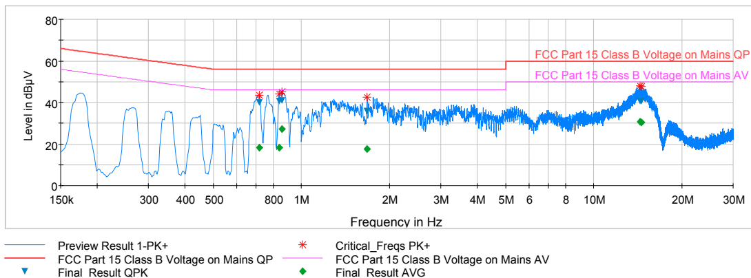
Plot 6-66. Line Conducted Plot with 802.11a (N)
