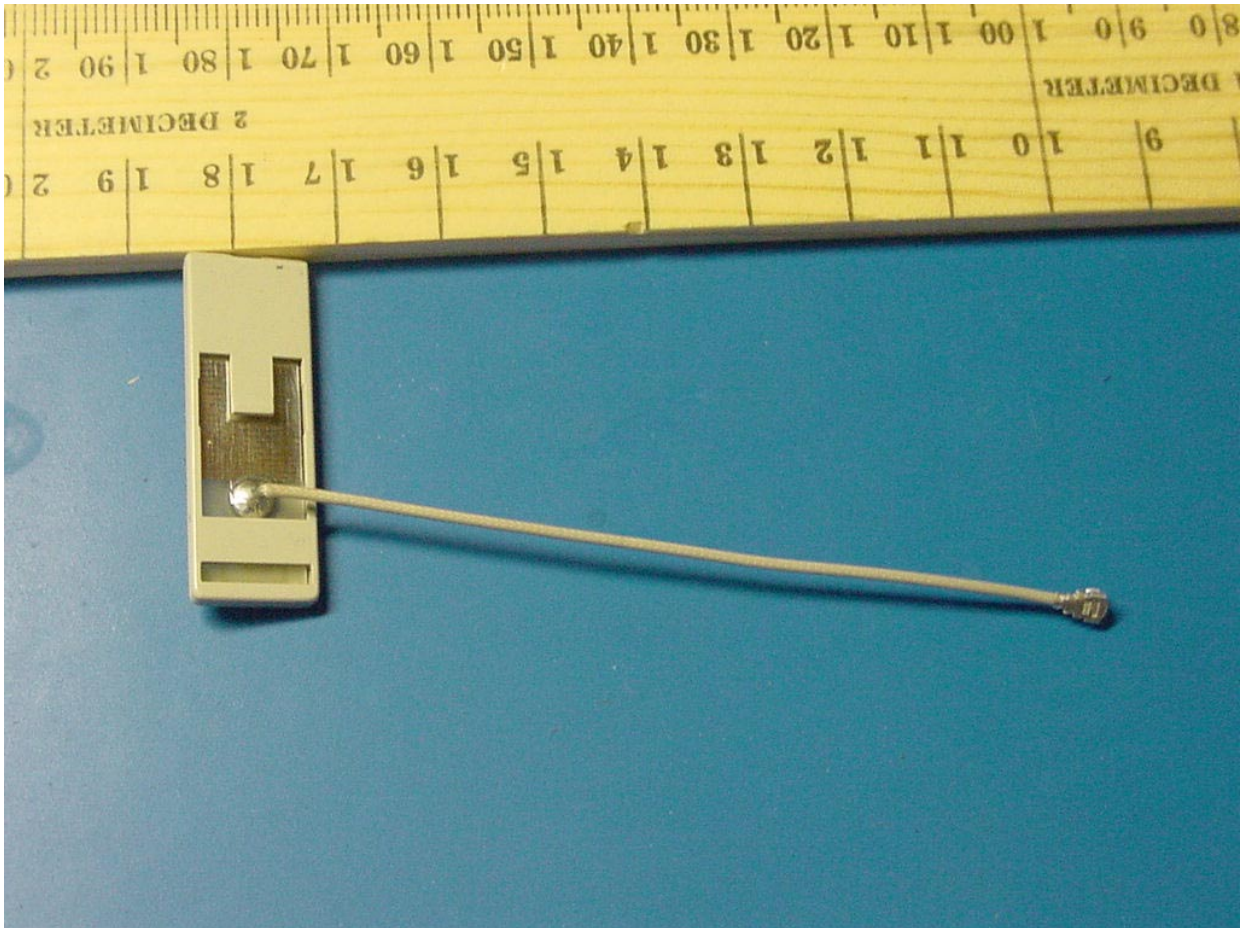
PHOTOGRAPH 13-10: WLAN ANTENNA BOTTOM
