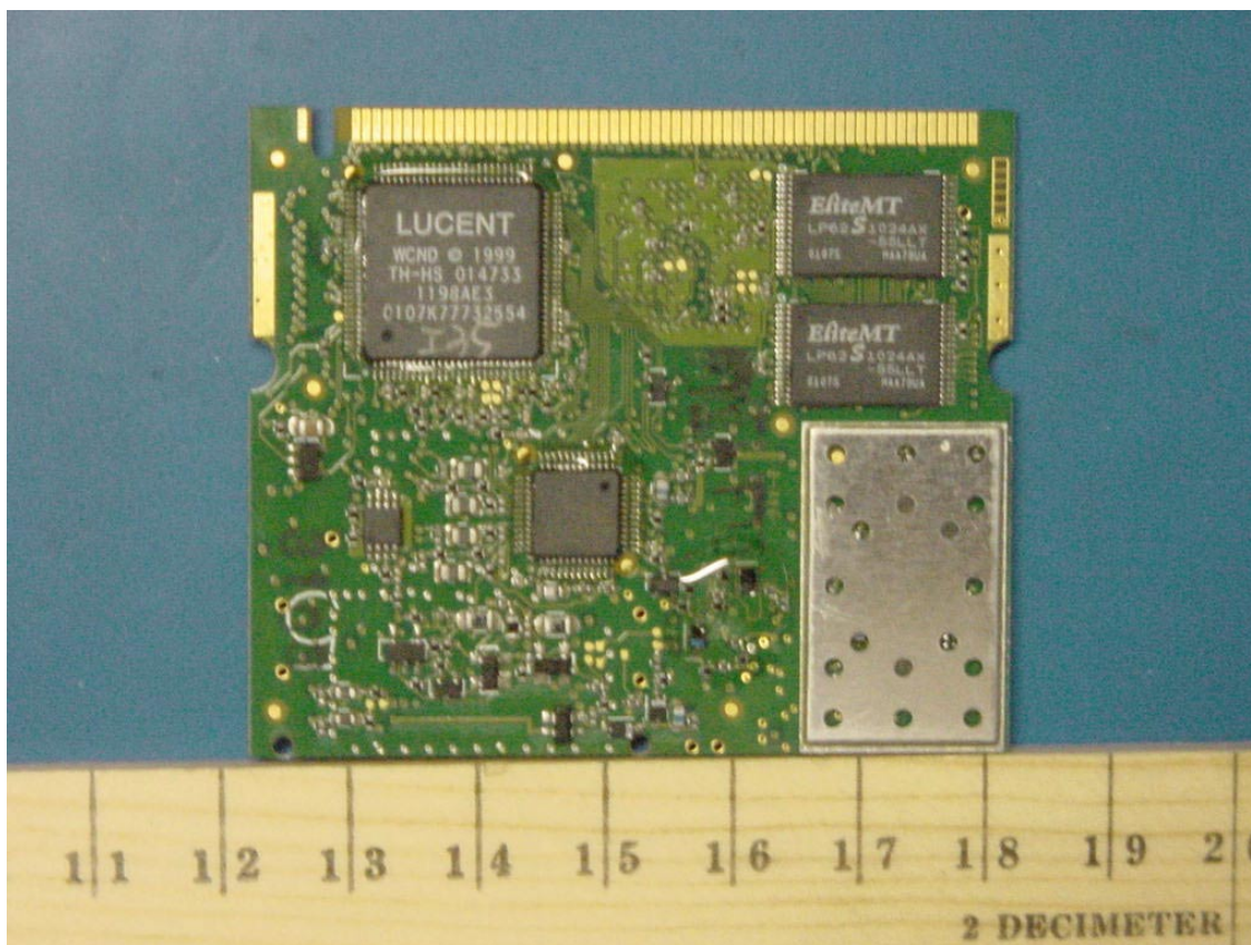
PHOTOGRAPH 13-6: BOTTOM VIEW
