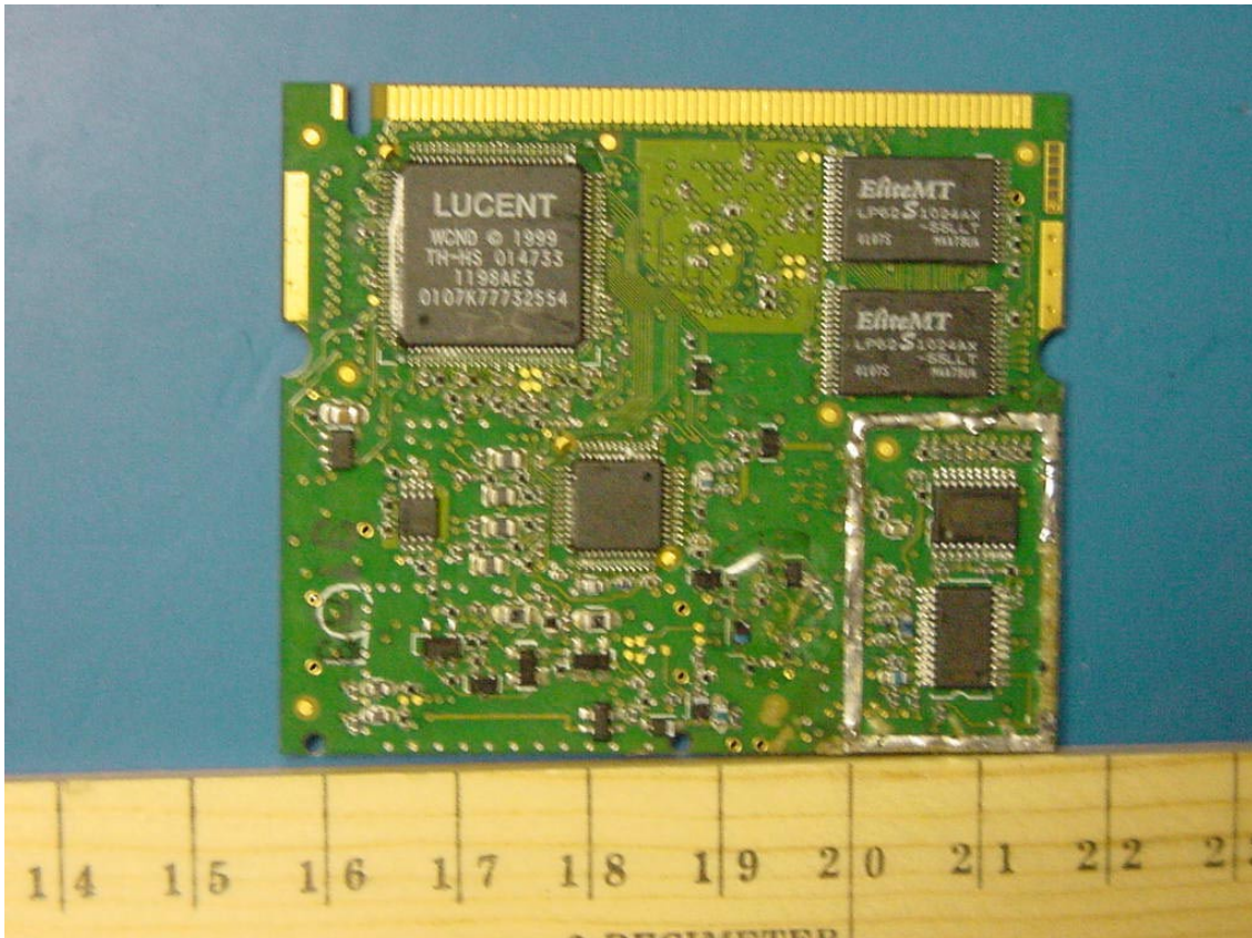
PHOTOGRAPH 13-8: BOTTOM VIEW OF THE BOARD WITHOUT CAN
