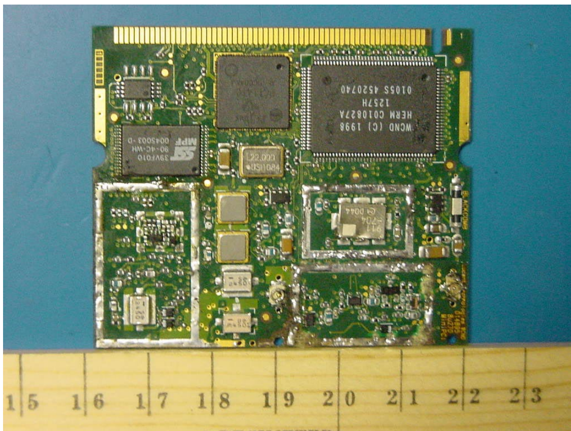
PHOTOGRAPH 13-7: TOP VIEW OF THE BOARD WITHOUT CAN
