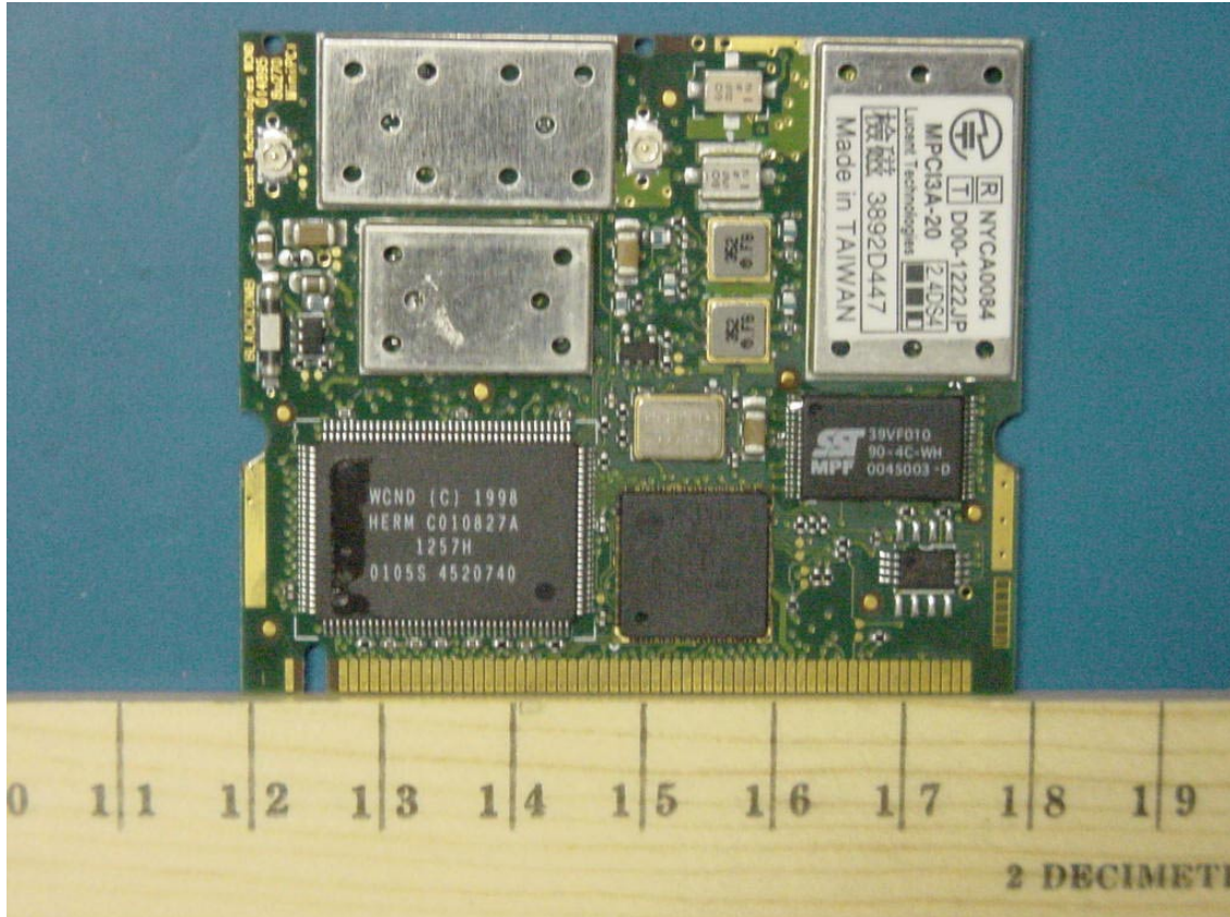
PHOTOGRAPH 13-5: TOP VIEW
