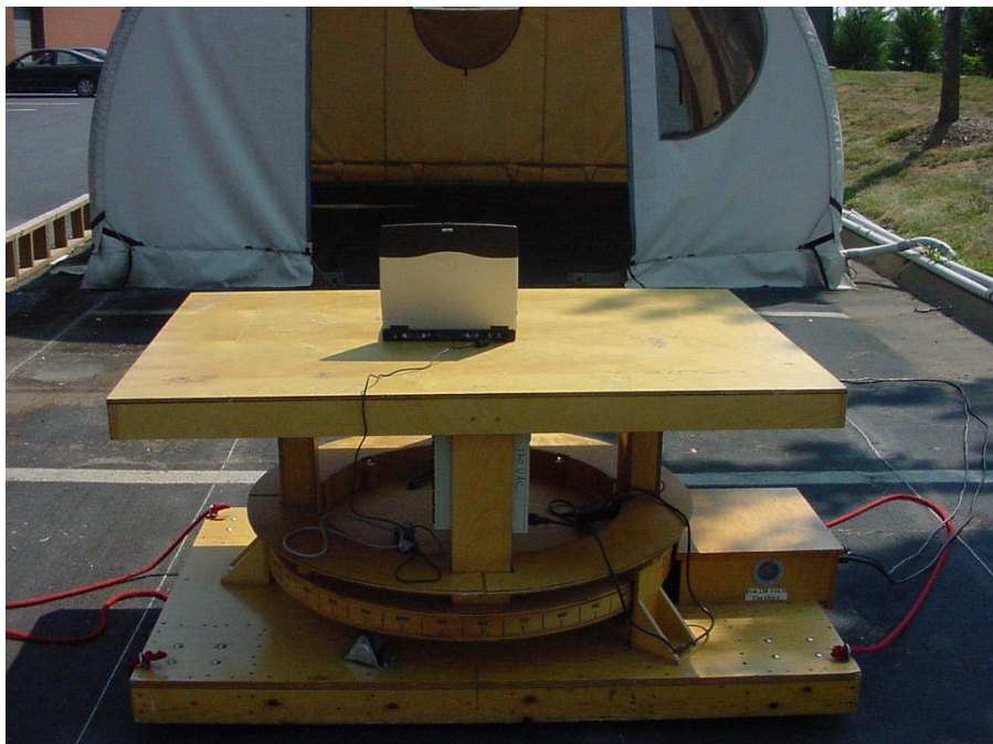
PHOTOGRAPH 13-4: RADIATED EMISSIONS REAR VIEW
