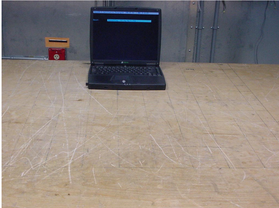
PHOTOGRAPH 13-1: CONDUCTED EMISSIONS FRONT VIEW
