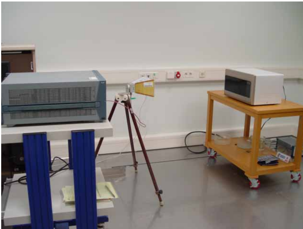
Fig. 4 Operating Frequency Measurements Configuration
