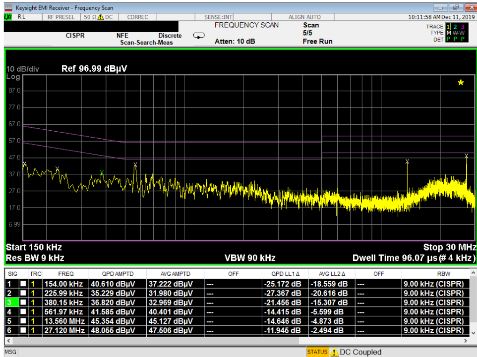
Plot 7-6. Line-Conducted Test Plot with Antenna (N)
