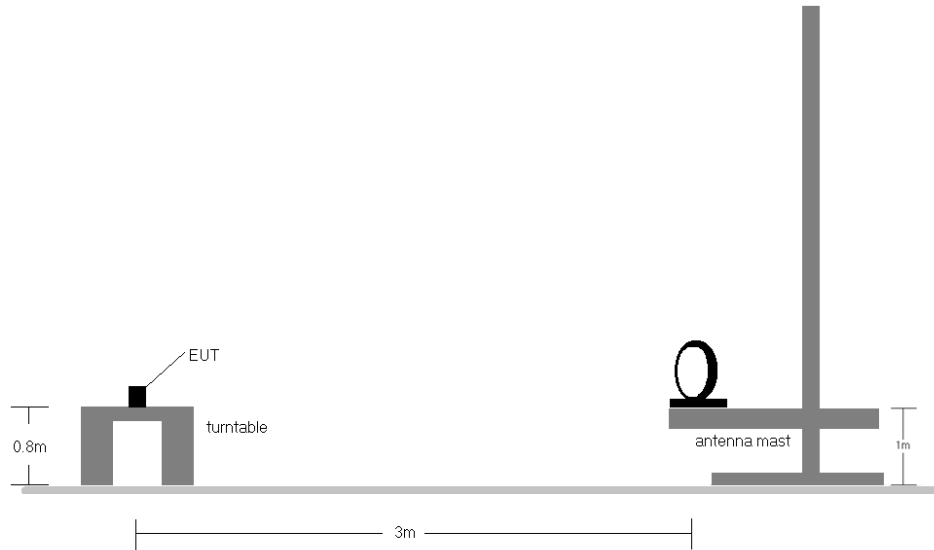
Figure 7-4. Radiated Test Setup
