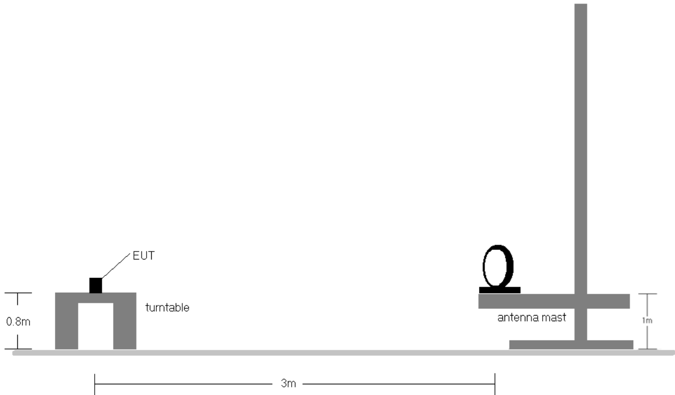
Figure 7-5. Radiated Test Setup < 30MHz
