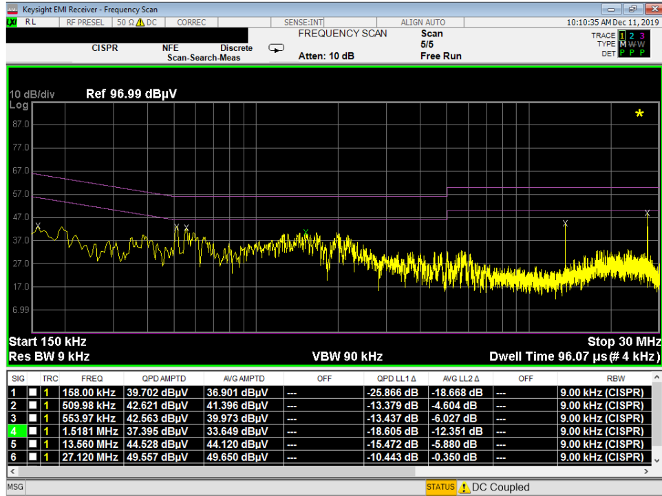
Plot 7-5. Line-Conducted Test Plot with Antenna (L1)
