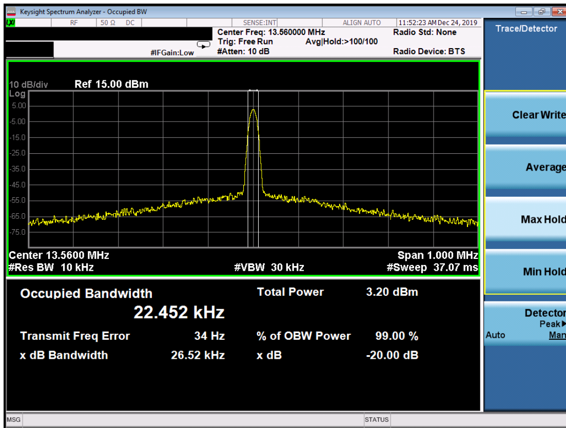
Figure 7-2. Occupied Bandwidth Plot
