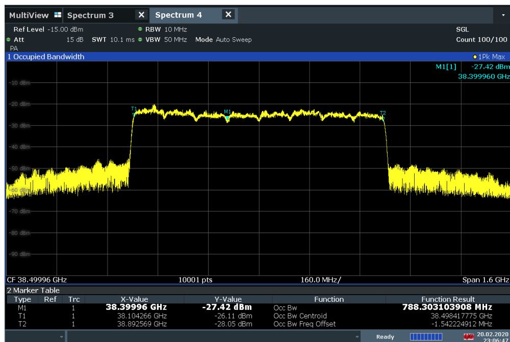
Plot 7-47. Occupied Bandwidth Plot (100MHz BW 8CC 16QAM Mid Channel)
