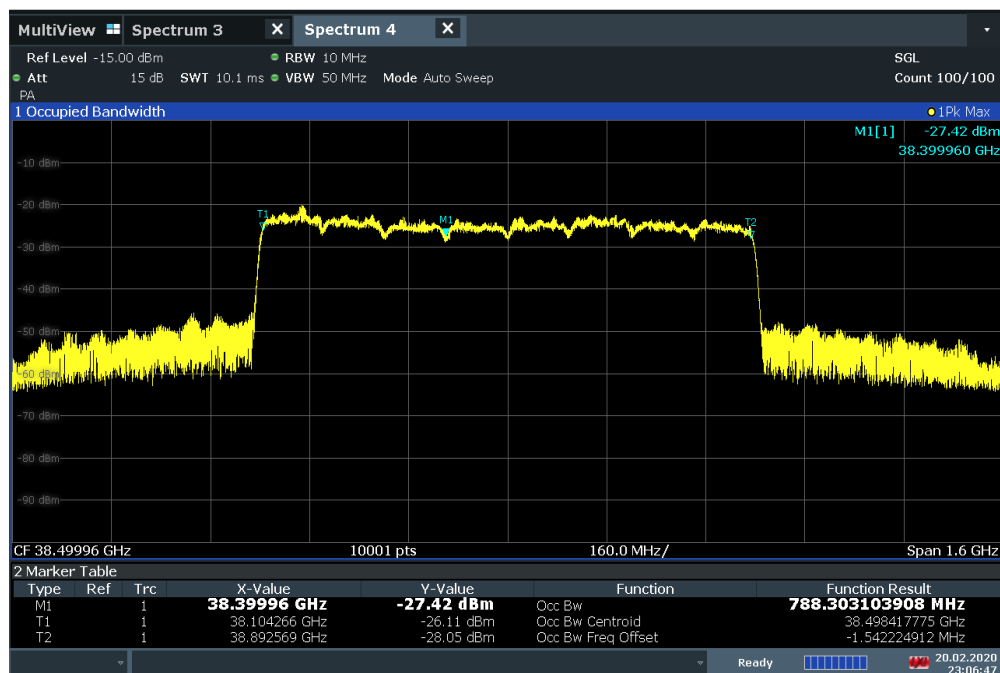
Plot 7-48. Occupied Bandwidth Plot (100MHz BW 8CC 64QAM Mid Channel)
