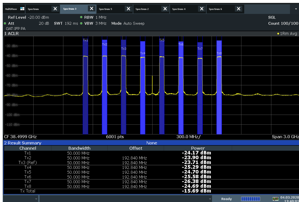
Plot 7-147. Antenna B EIRP Density Plot (50MHz BW 8CC NC 64QAM Mid Channel)
