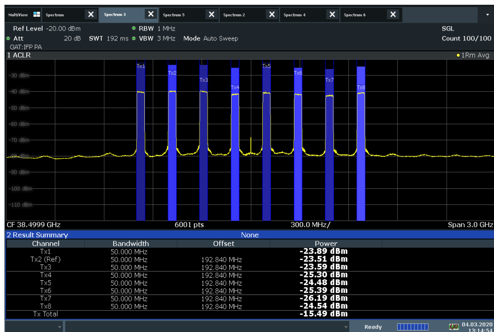
Plot 7-91. Antenna A EIRP Density Plot (50MHz BW 8CC NC QPSK Mid Channel)
