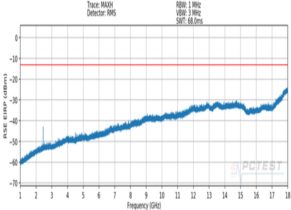
Plot 7-290. RSE 1 GHz – 18 GHz (100 MHz BW 4CC CC QPSK Low Ant. Pol. V)
