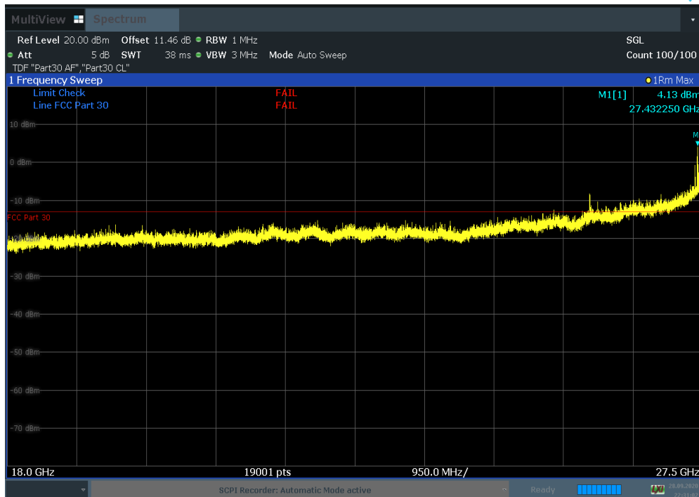
Plot 7-358. RSE 18 GHz – 27.5 GHz (100 MHz BW 8CC CC QPSK Mid Ant. Angle 45)
