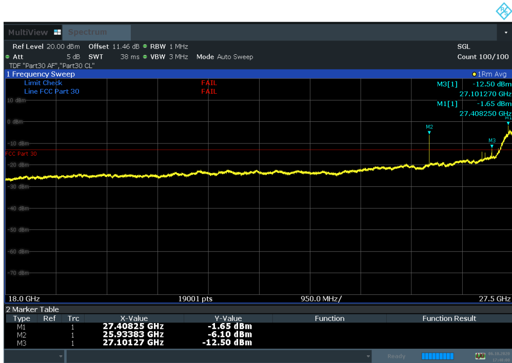
Plot 7-316. RSE 18 GHz – 27.5 GHz (100 MHz BW 4CC CC QPSK Low Ant. Angle 135, Final)
