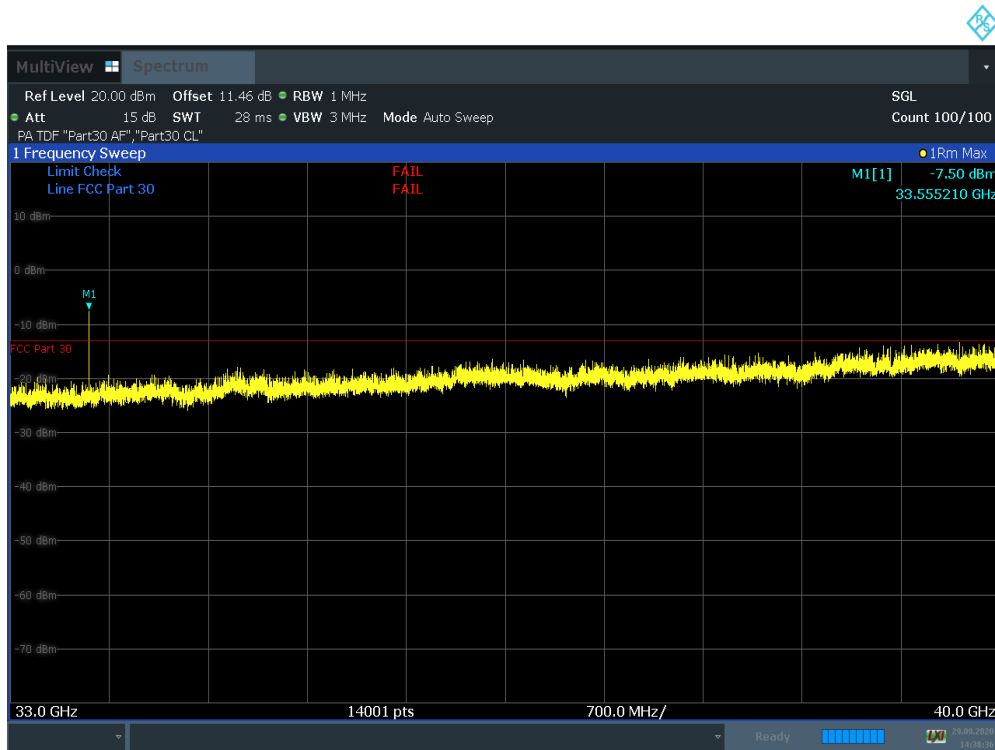
Plot 7-576. RSE 33 GHz – 40 GHz (50 MHz BW 2CC + 100 MHz BW 3CC NC QPSK Mid Ant. Angle 135)
