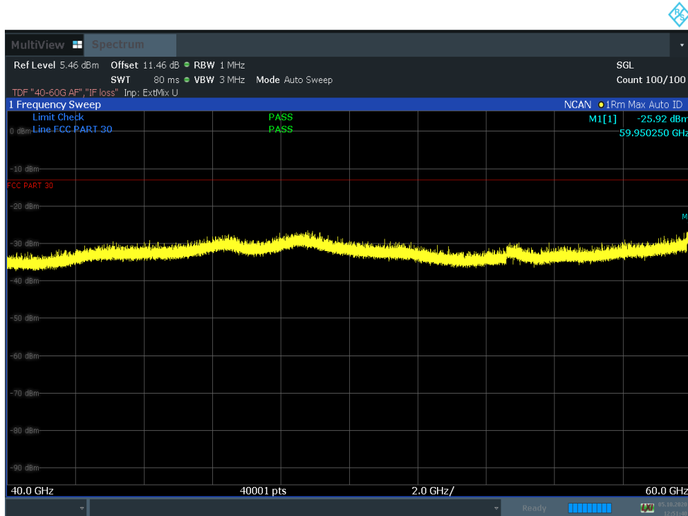
Plot 7-639. RSE 40 GHz – 60 GHz (100 MHz BW 4CC CC QPSK High Ant. Pol. V)
