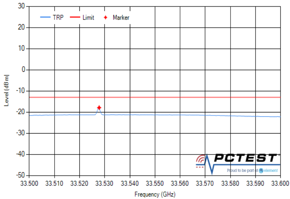
Plot 7-621. RSE 33.5 GHz – 33.6 GHz (50 MHz BW 2CC + 100 MHz BW 6CC NC QPSK High TRP)
