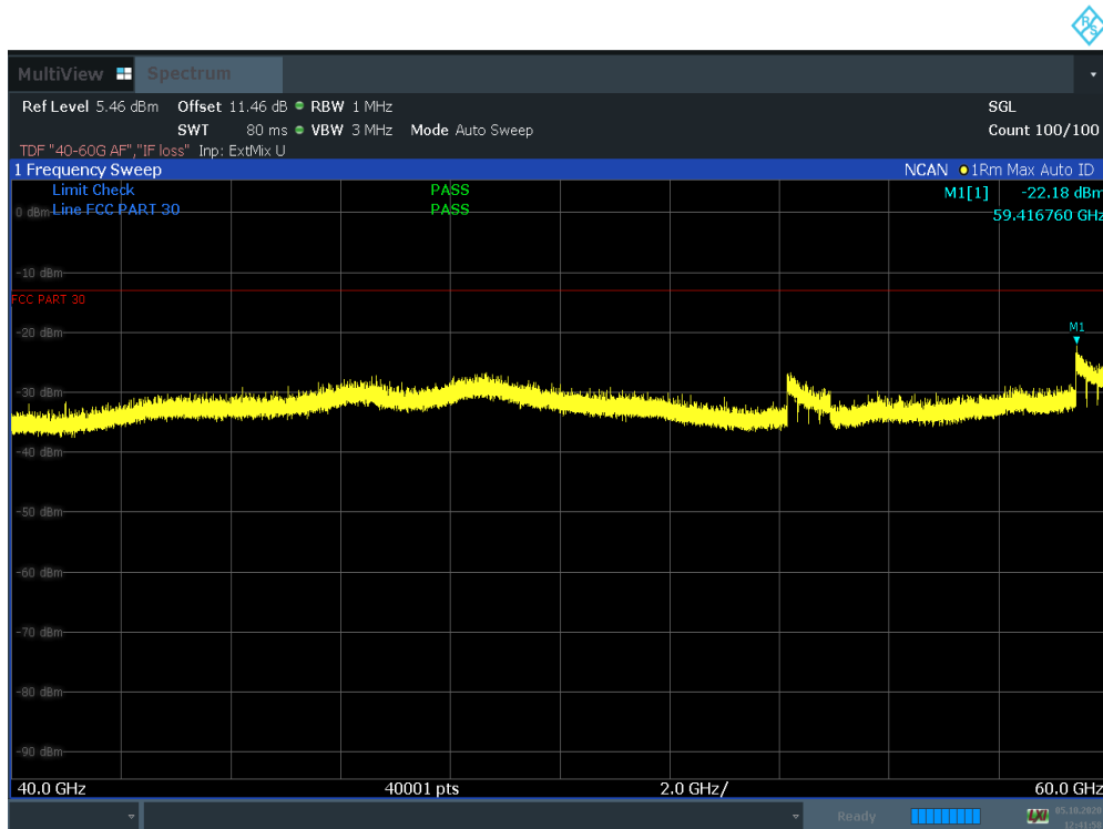
Plot 7-631. RSE 40 GHz – 60 GHz (100 MHz BW 4CC CC QPSK Mid Ant. Pol. V)
