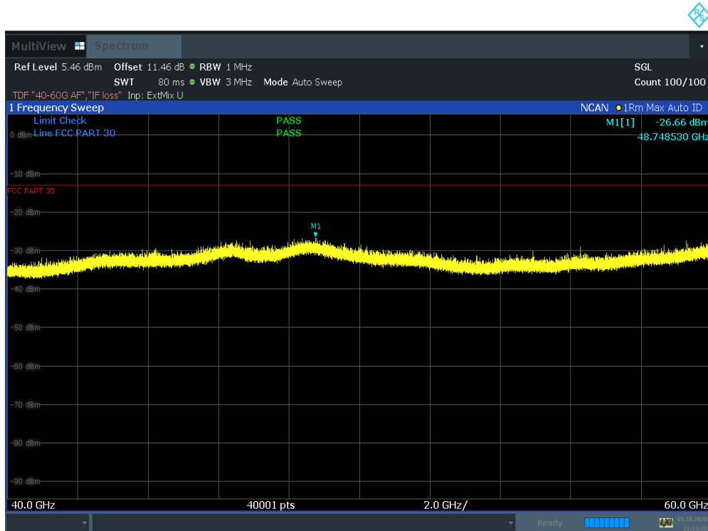
Plot 7-633. RSE 40 GHz – 60 GHz (100 MHz BW 8CC CC QPSK Mid Ant. Pol. V)
