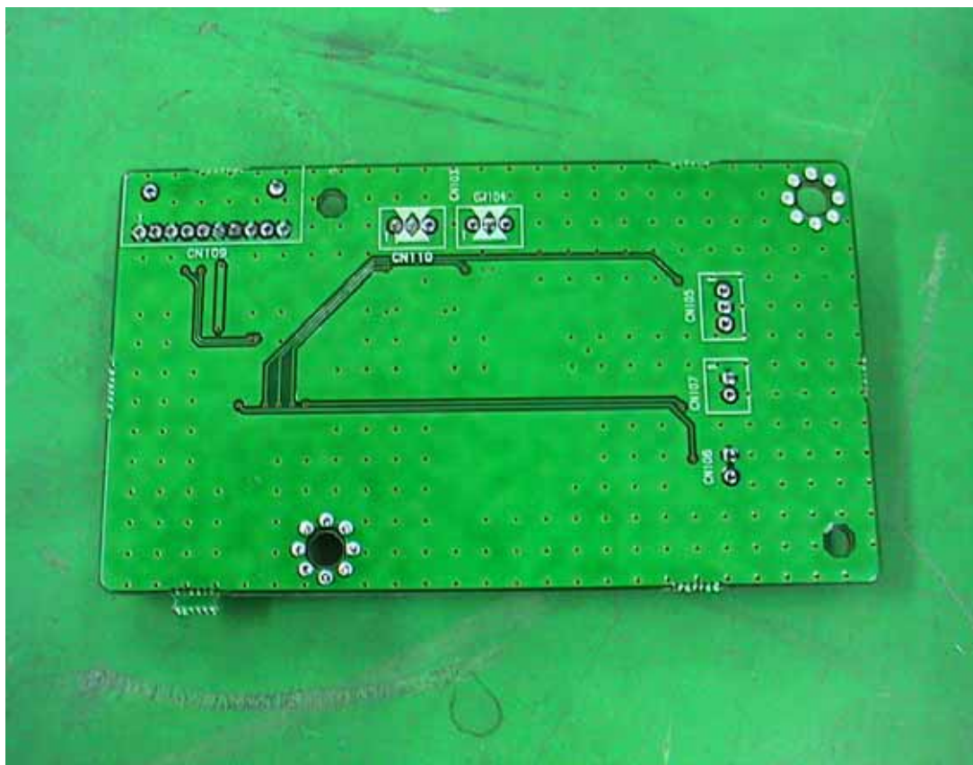
Sub detect board bottom view
