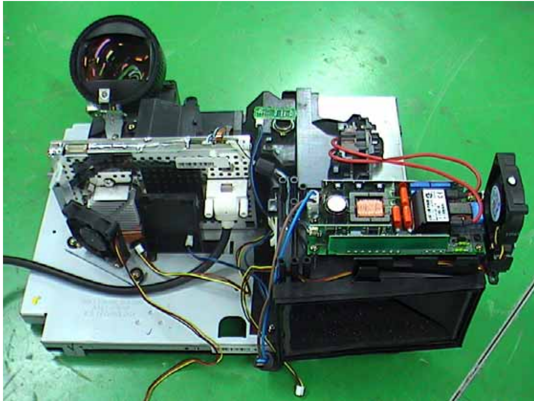
Engine view
