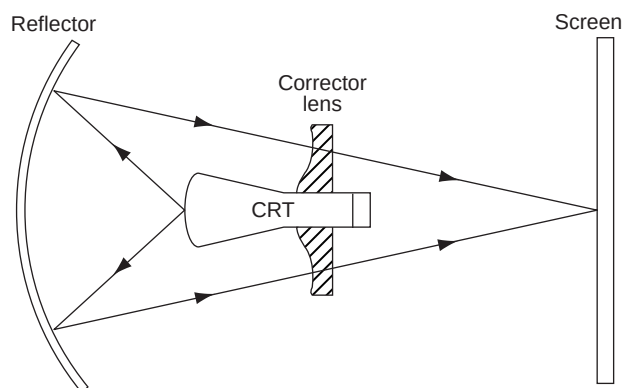
Figure 4. CRT projection system with Schmidt optics. 4
