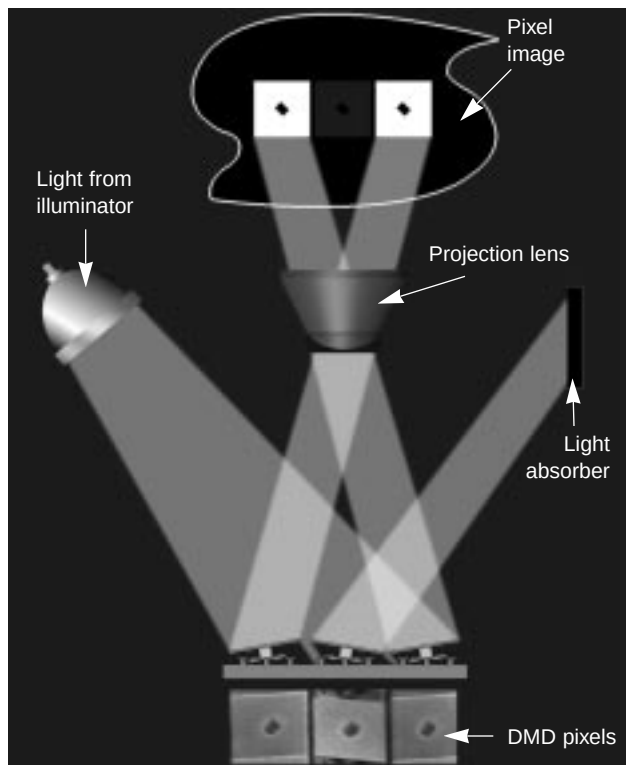
Figure 2. Dark field projection of a DMD.
