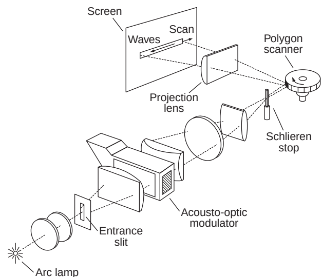
Figure 7. Scophony projection system (vertical scanner not shown). 12
