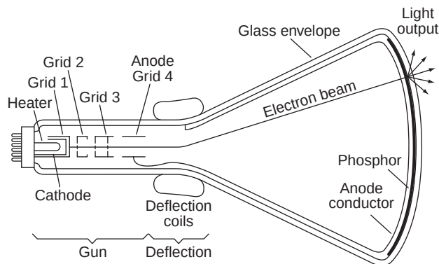
Figure 8. Magnetically deflected CRT. 14
