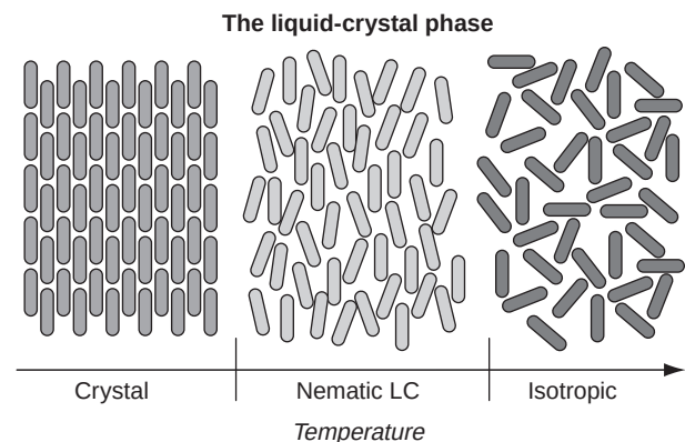
Figure 17. The phases of a nematic liquid crystal as a function of temperature. 46
