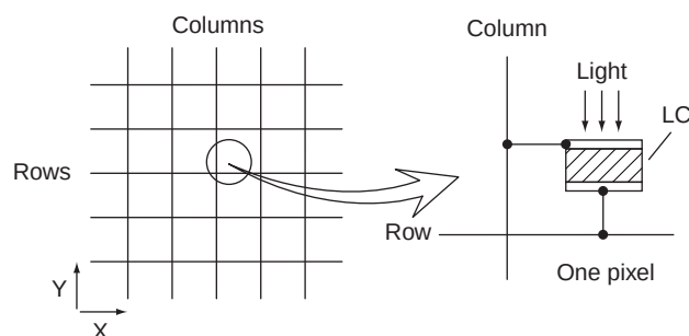
Figure 25. Passive-matrix address method.
