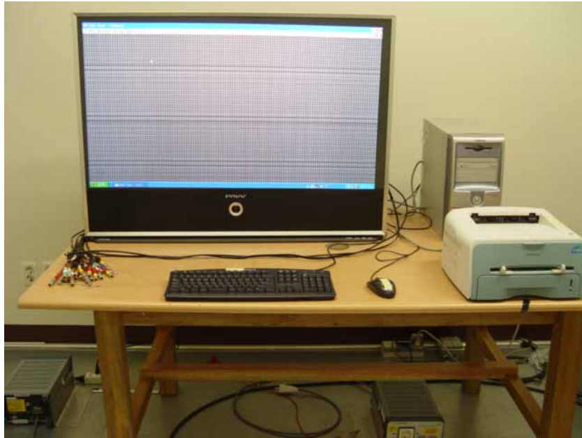
Pic. 1 Conducted Emission (Front)
