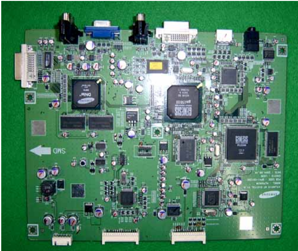
Digital board top view
