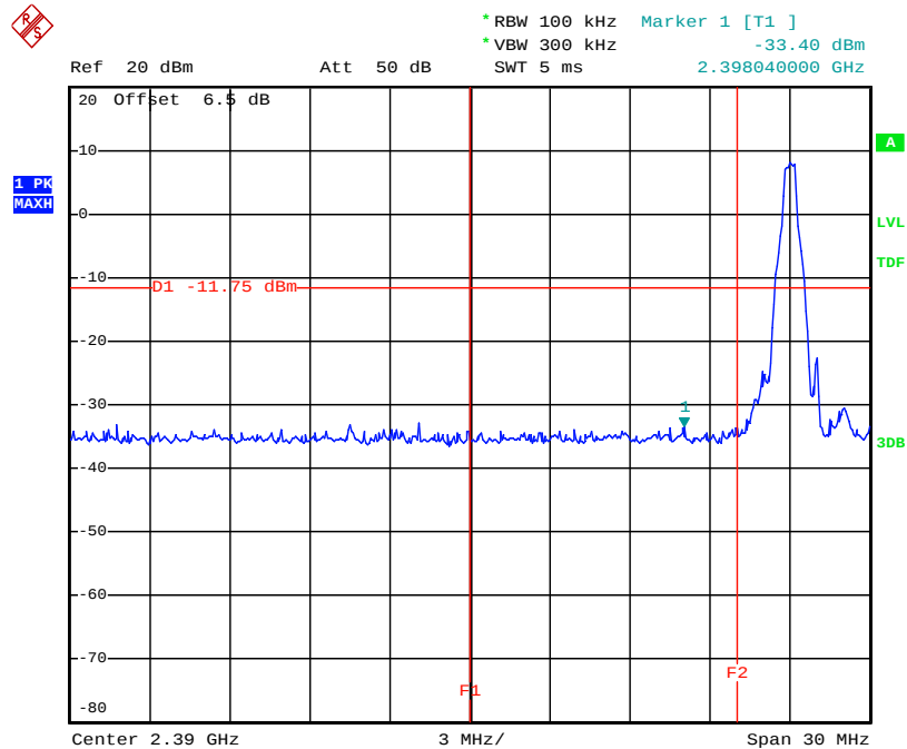
Figure 6. Plot of the Band Edge (Conducted)
