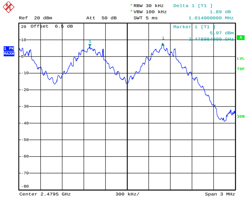
Figure 2. Plot of the Carrier Frequency Separation (Conducted)
