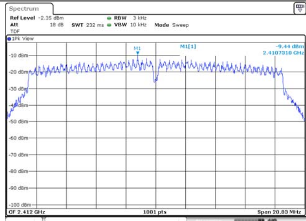
802.11n HT20 / 2 412 MHz
