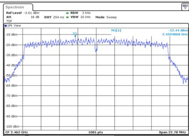
802.11n HT20 / 2 462 MHz
