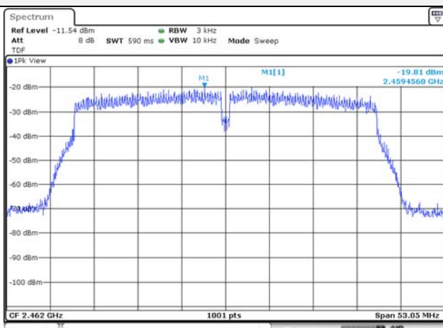
802.11n HT40 / 2 462 MHz
