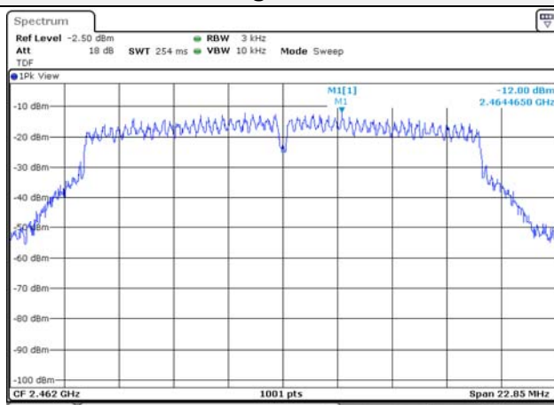
802.11g / 2 462 MHz
