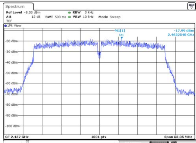
802.11n HT40 / 2 457 MHz
