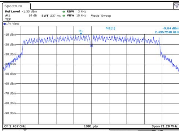
802.11g / 2 437 MHz
