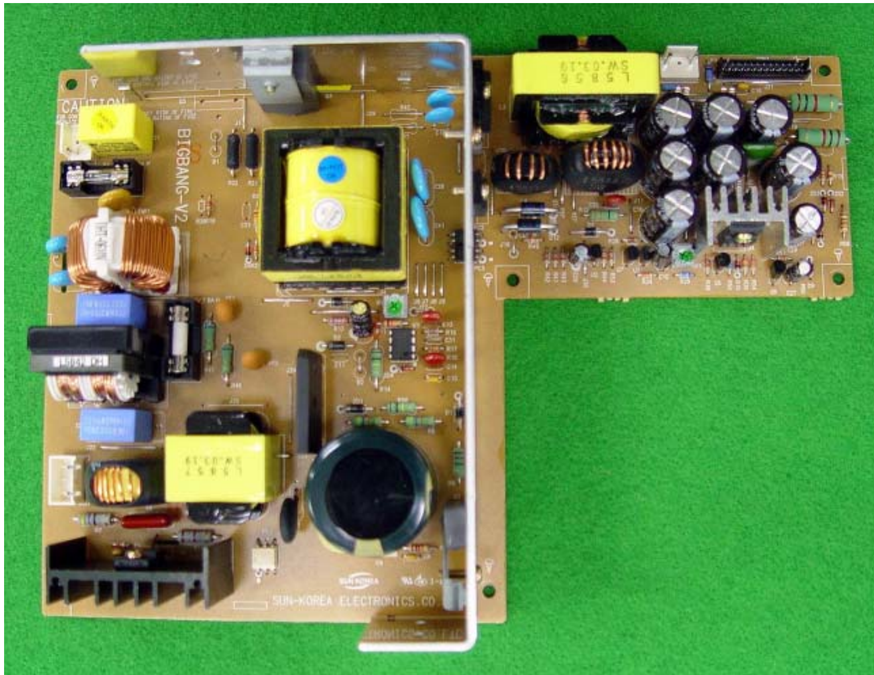
SMPS Board TOP
