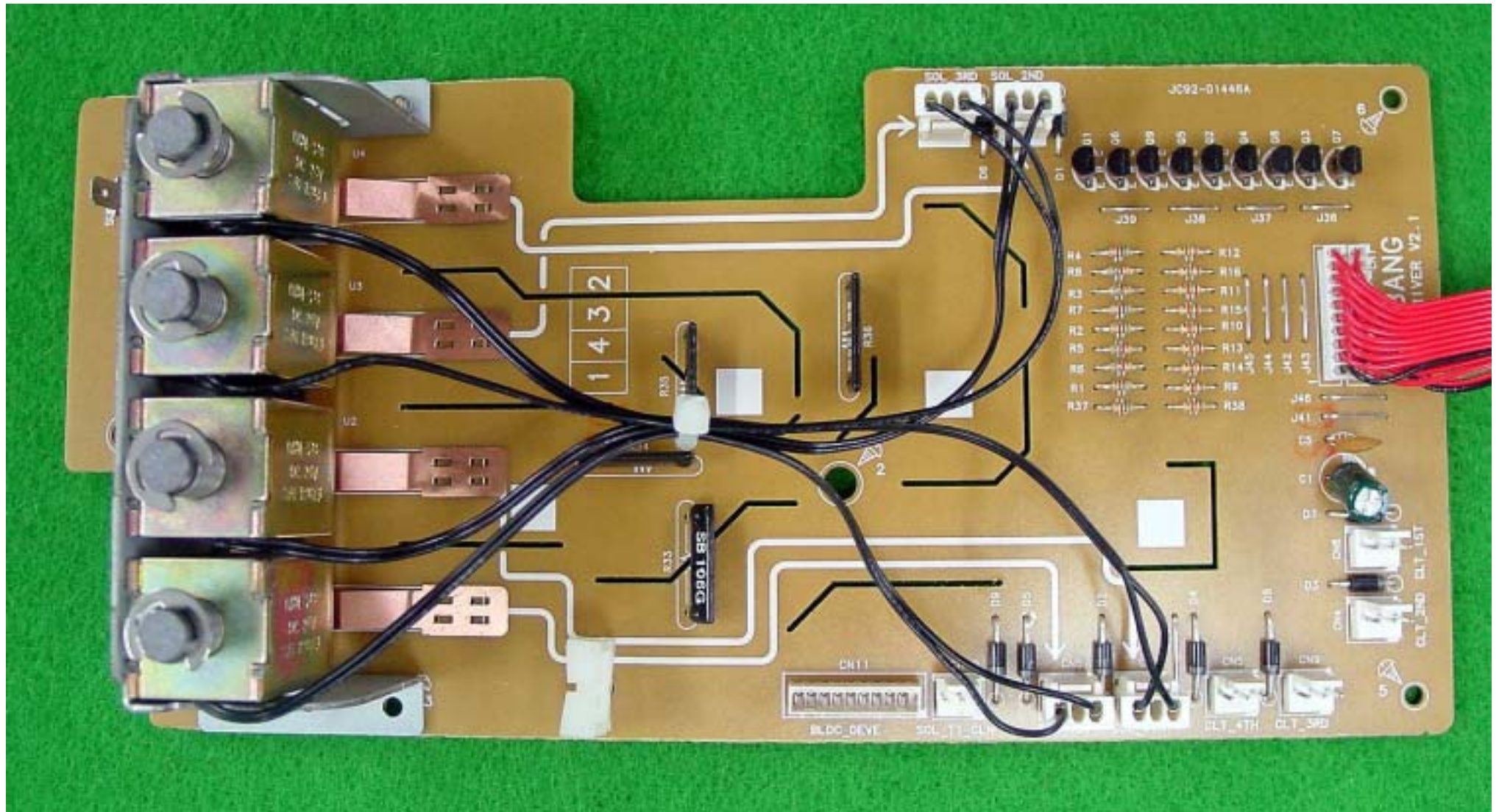
DEV_Switch Board TOP
