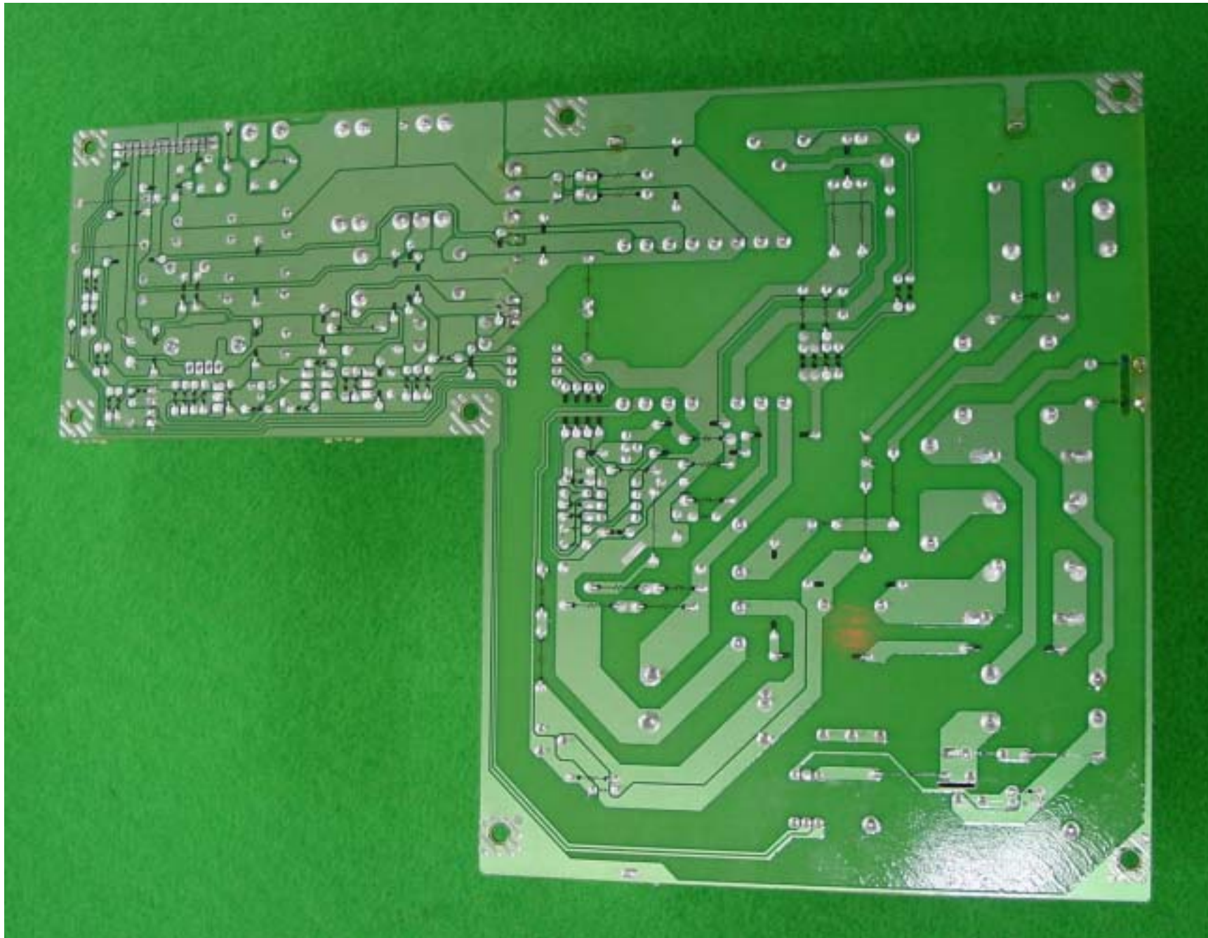
SMPS Board BOTTOM
