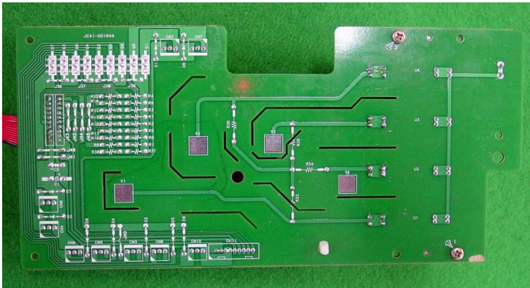
DEV_Switch Board BOTTOM
