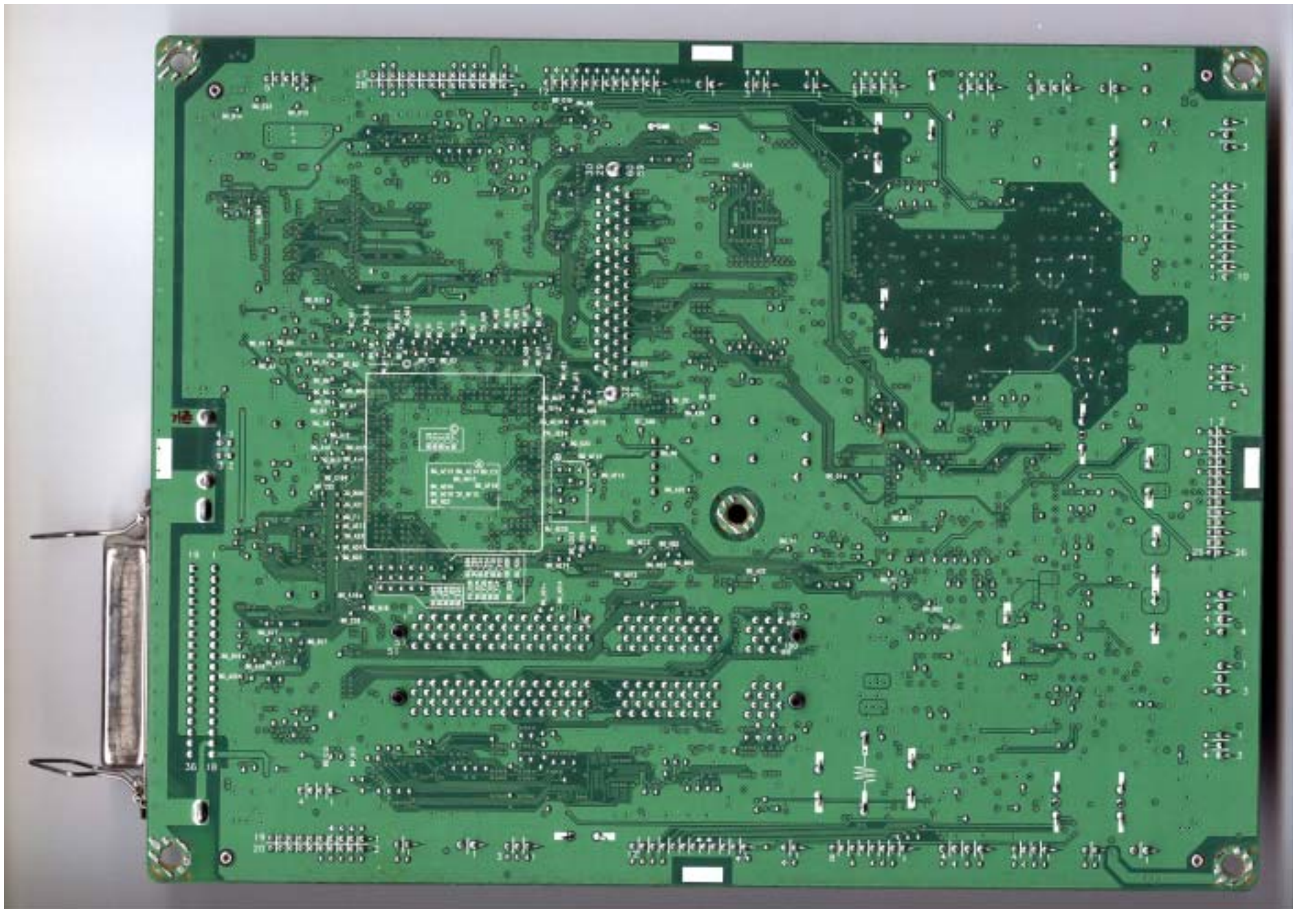
MAIN Board BOTTOM
