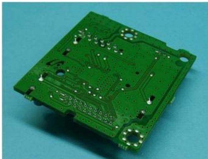
10) Bottom View of ADF Joint (CLX-3185FN/FW))
