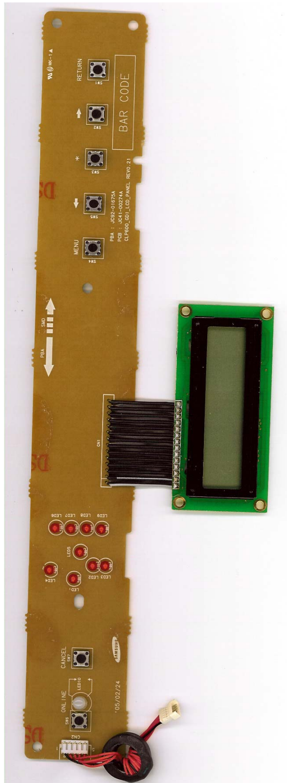
Fig. 07 Panel PBA
