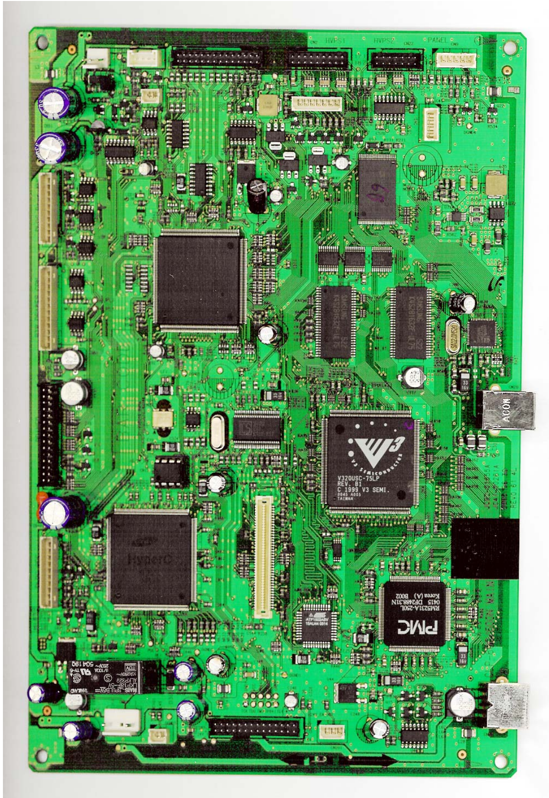
Fig. 01 Main PBA
