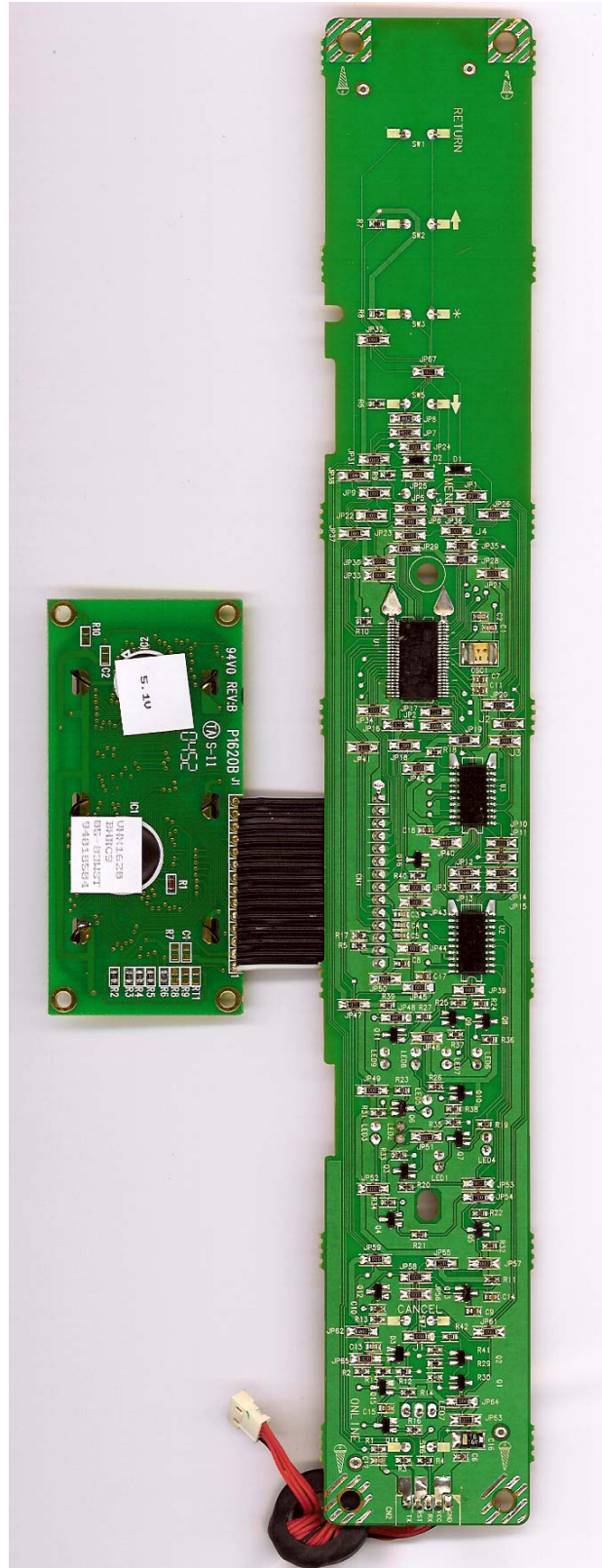
Fig. 08 Panel Solder
