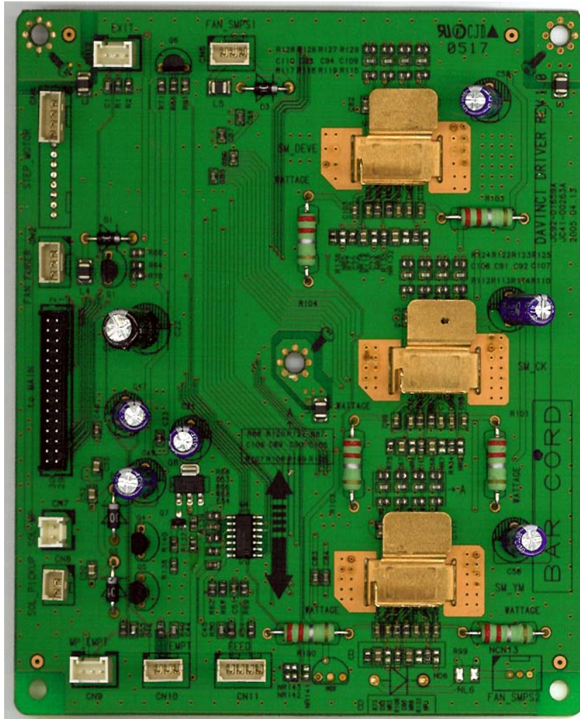
Fig. 09 Driver PBA
