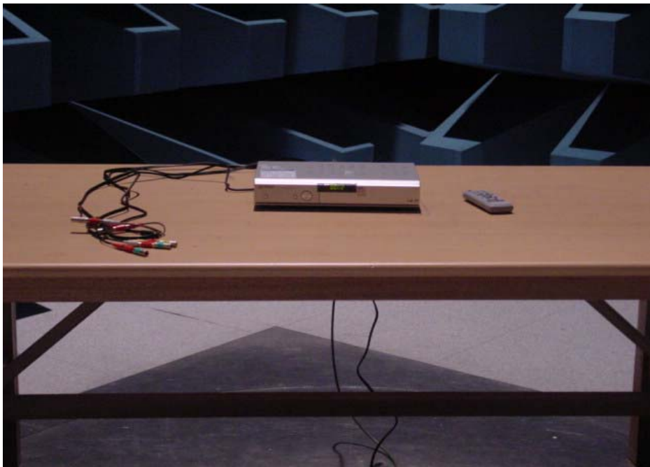
Picture 4. Radiated Emission (Front)
