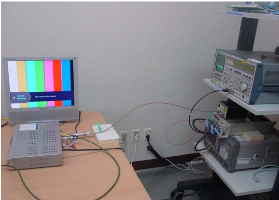
Picture 6. Output Signal Level
