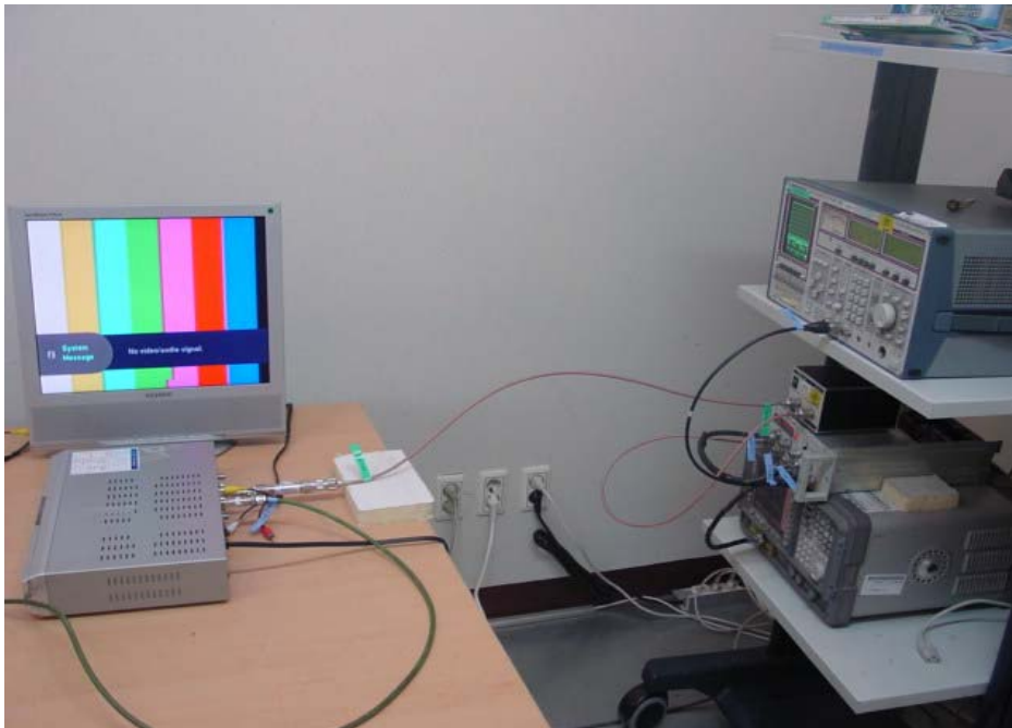
Picture 7. Output Terminal Conducted Spurious Emission
