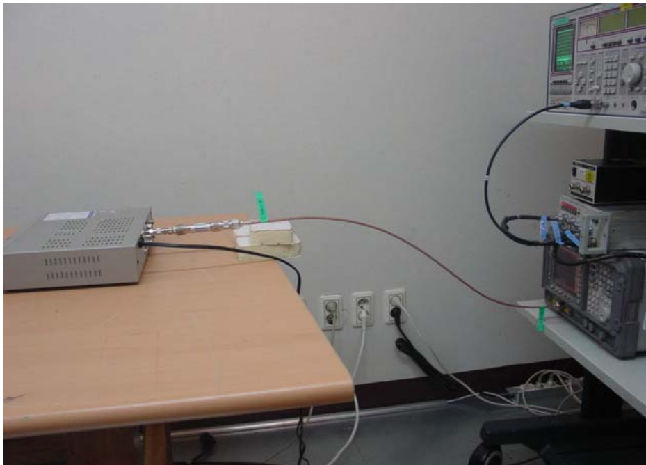
Picture 3. Antenna Terminals
