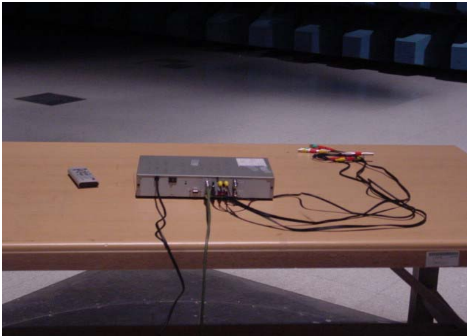
Picture 5. Radiated Emission (Rear)
