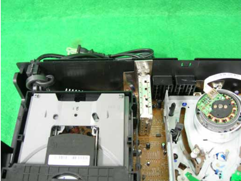
METAL SHIELD/FERRITE CORE VIEW
