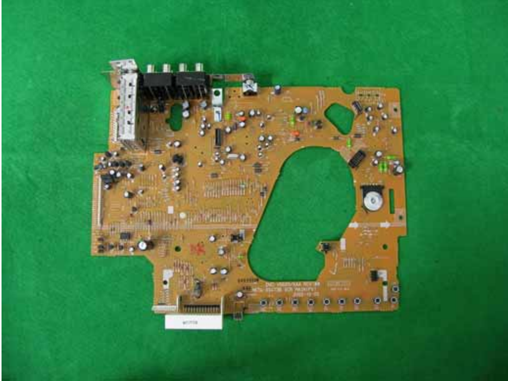
TOP of MAIN PCB VIEW
