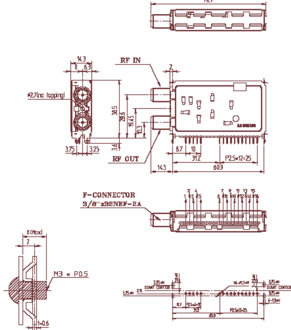
Dimension of P.C.B for Tm-Block Mounting (Viewed from Copper Pattern)
