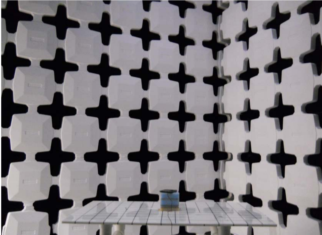
Figure 3 Radiated Test Setup
