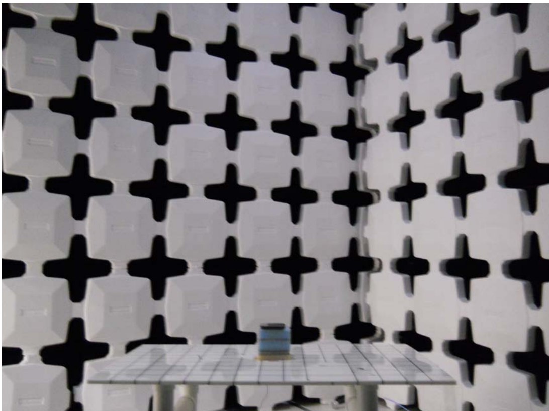
Figure 4 Radiated Test Setup
