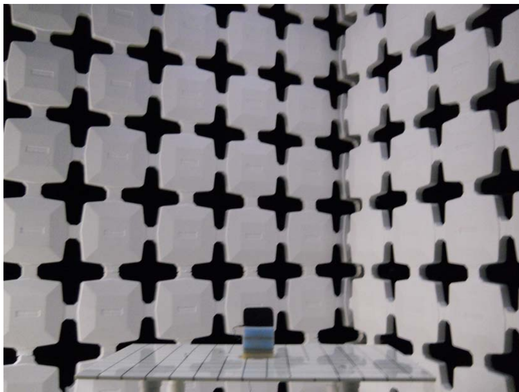
Figure 5 Radiated Test Setup
