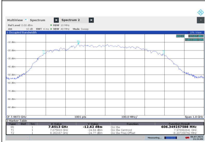
SP0_BPRF 20_Preamble 12
