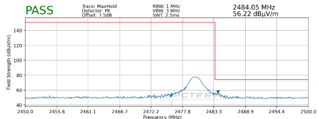
Plot 7-25. Radiated Restricted Upper Band Edge Measurement (Peak)
