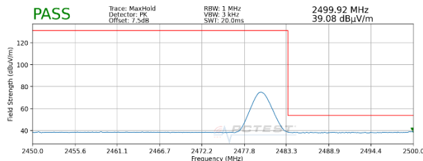
Plot 7-24. Radiated Restricted Upper Band Edge Measurement (Average)
