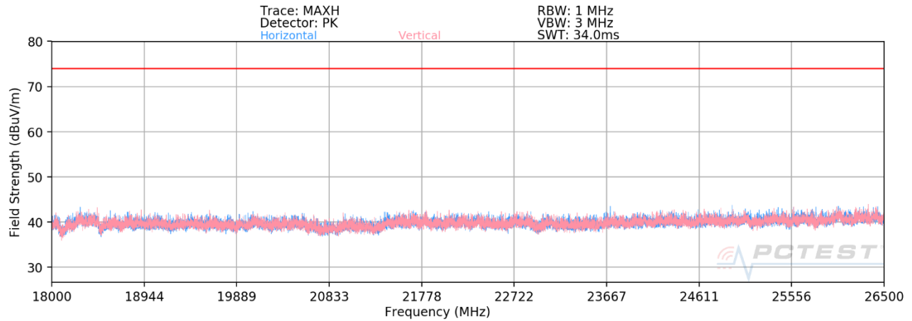
Plot 7-21. Radiated Spurious Plot above 18GHz
