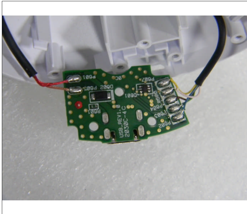
Bottom view of sub board #3
