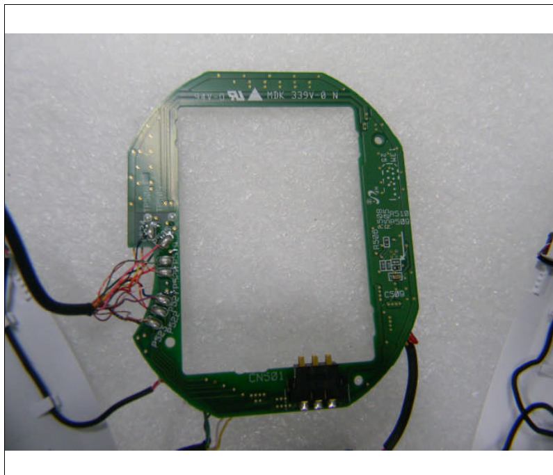
Bottom view of sub board #1
