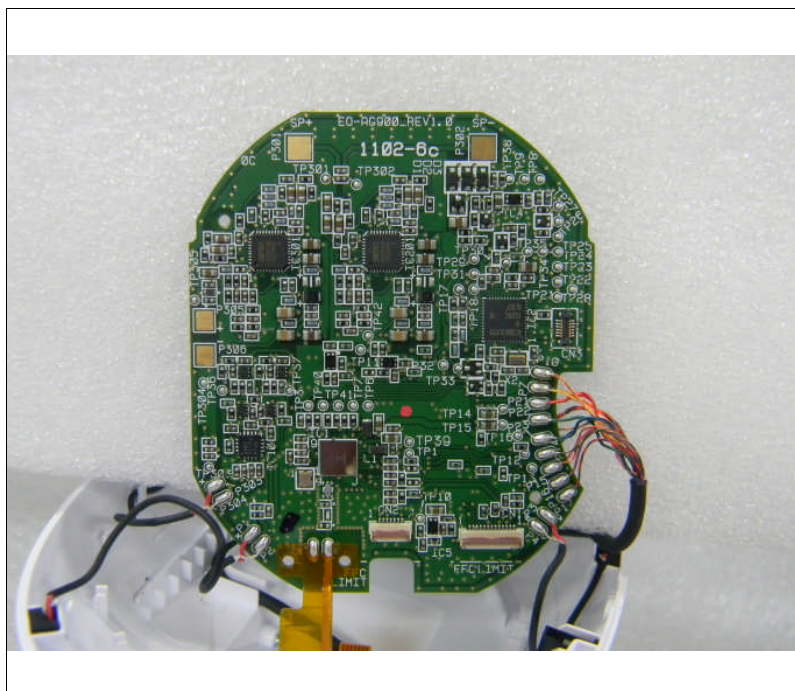
Bottom view of main board
